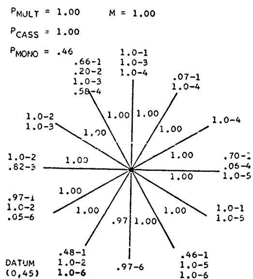
ENVIRONMENT: NORTH ATLANTIC LAYER DEPTH (FT): 150 SYSTEM: SJS-26/CASS XMTF MODE: EL/ODT, DP TARGET DEPTH (FT): 300 TARGET SPEED (KNOTS): 10 SHIP SPEED (KNOTS): 15 AIRCRAFT SPEED (KNOTS): 120 BUOY DEPTHS (FT): 1500
