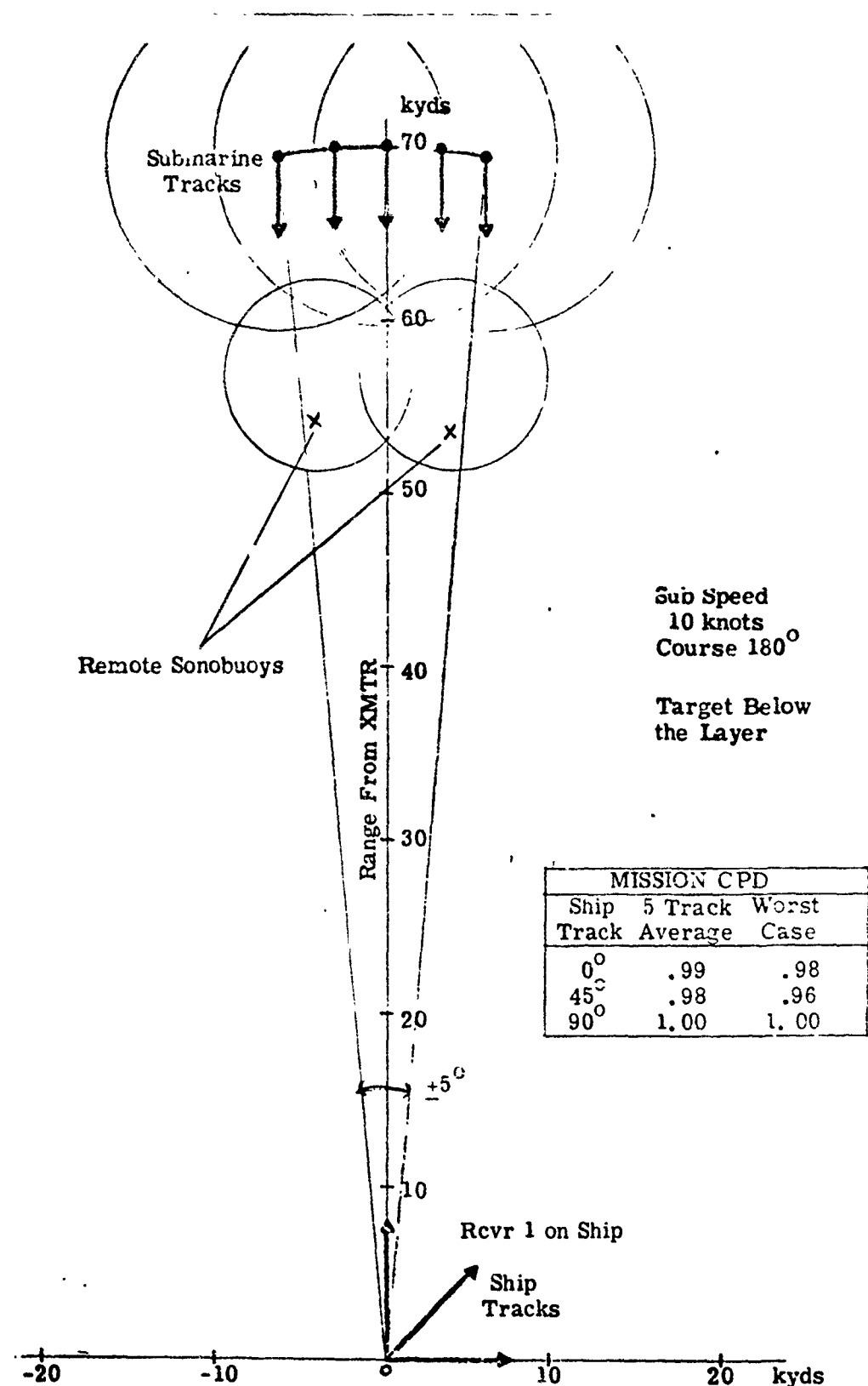
Figure 4-6 (C) Convoy Screening Scenario - Target Heading 180° Datum at 0°
