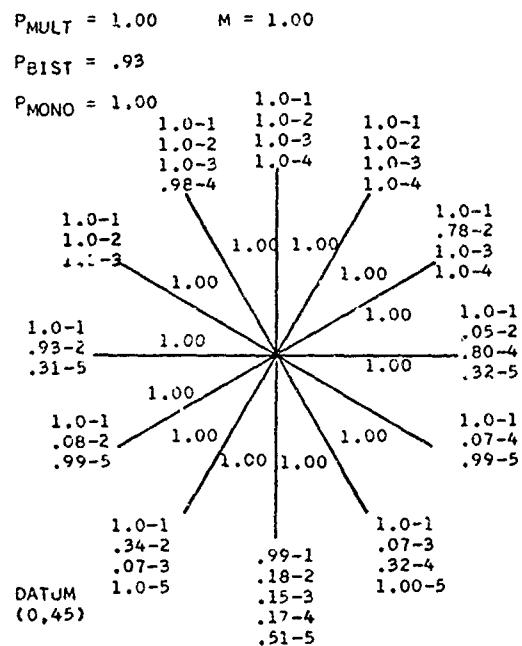
ENVIRONMENT: MEDITERRANEAN LAYER DEPTH (FT): (NO SURFACE DUCT) SYSTEM: SQS-26/41-A XMTF CODE: F-CDT TARGET DEPTH (FT): 300 TARGET SPEED (KNOTS): 10 SHIP SPEED (KNOTS): 15 AIRCRAFT SPEED (KNOTS): 120 BUOY DEPTHS (FT): 1500
