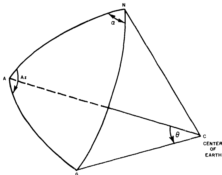
(U) Fig. 3 -- Spherical triangle NAG, where N is the North Pole, A is the navigator's assumed position, and G is the geographical position of the satellite. The arcs AN and NG are the colatitudes of the navigator and the satellite G, respectively.
