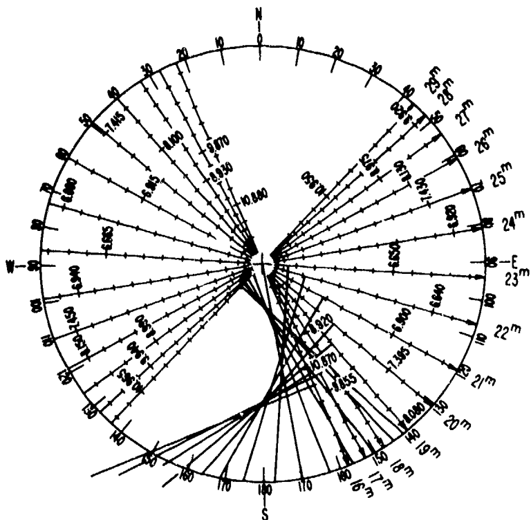
(U) Fig. 6 -- Intercept chart showing effect of clock synchronization error on plot
