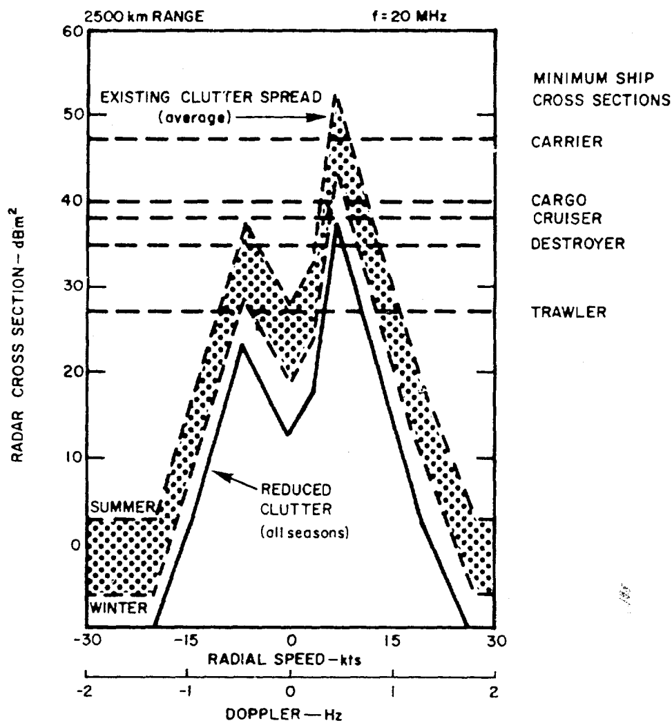
(S) Fig. 1 - Comparison of current and future sea-clutter-spectrum magnitudes with the expected minimum ship-cross-section magnitudes (reproduced from page 83 of Ref. 5)
