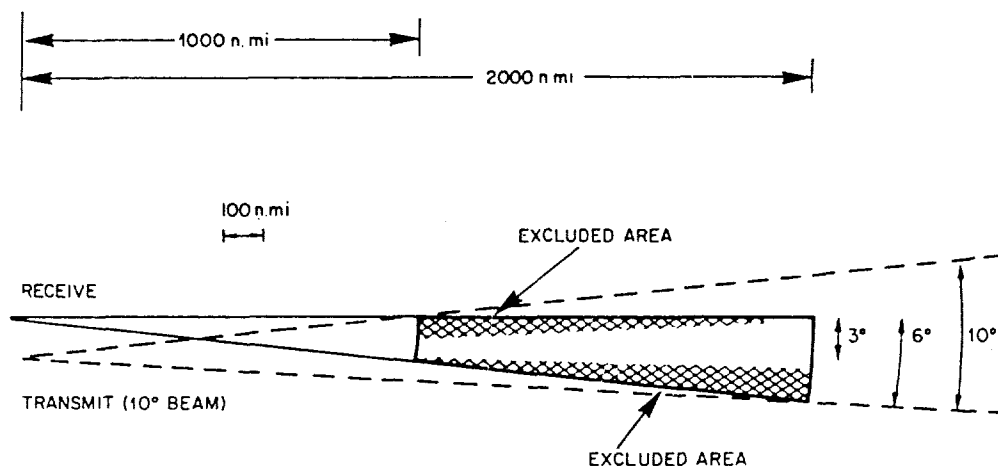
(S) Fig. 3—Geometry of a bistatic configuration
