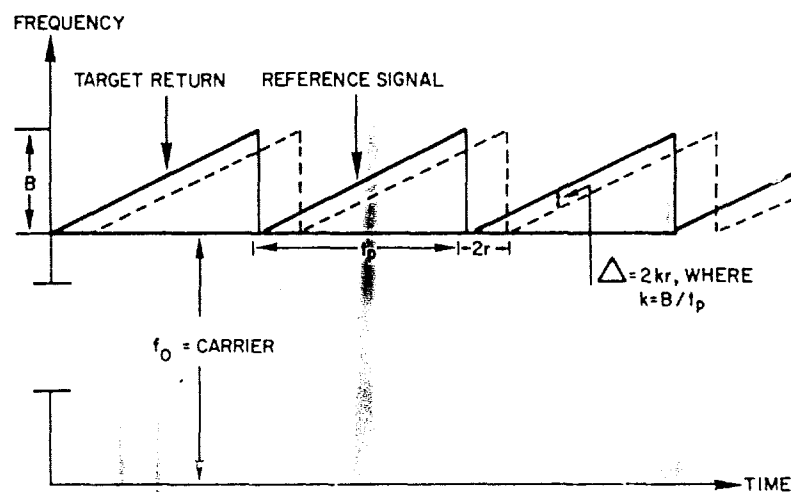
(S) Fig. 6—Relationship of range delay 2r and frequency difference \Delta
