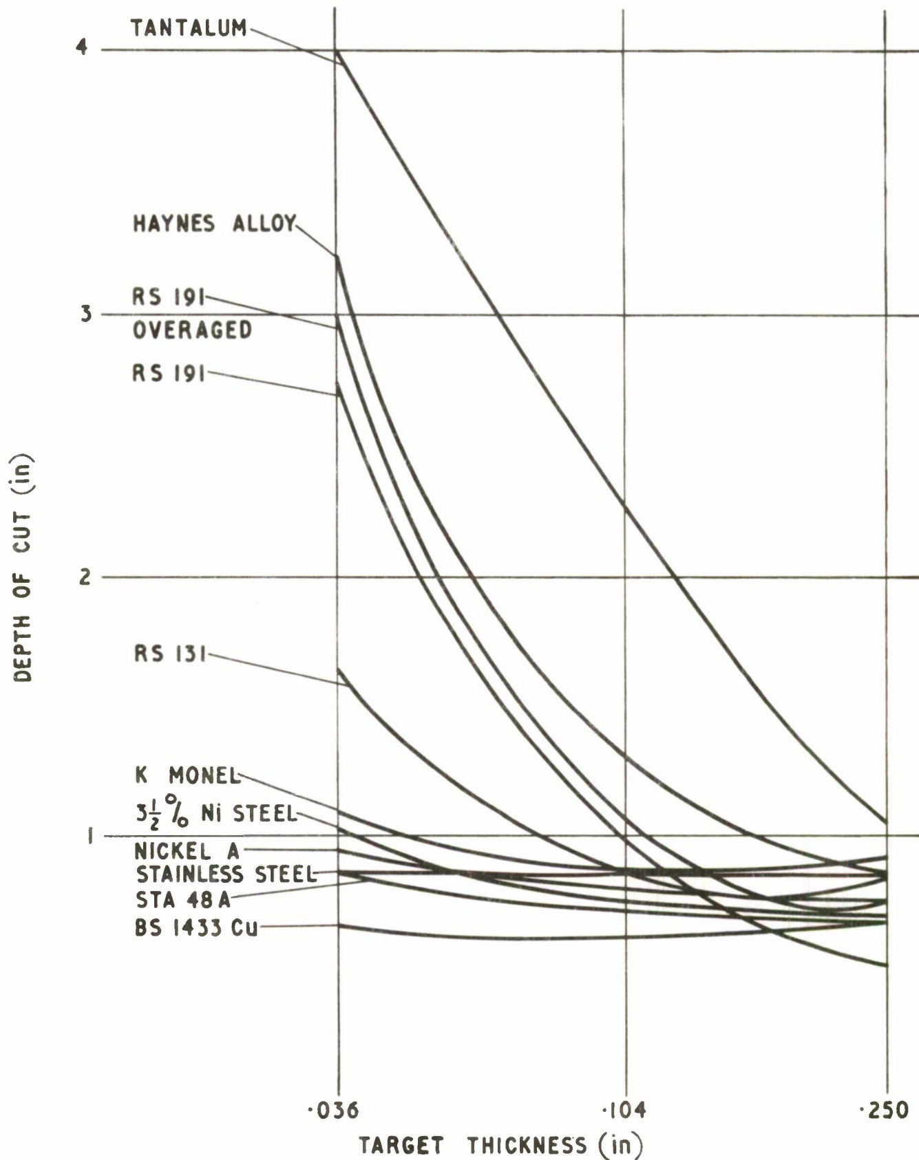
FIG. 8 DEPTHS OF CUT IN ALUMINIUM ALLOY TARGETS FROM HIGH VELOCITY RODS
