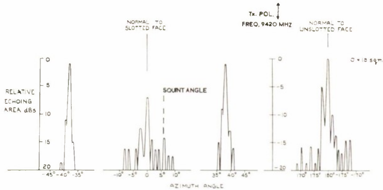
FIG. 3. Re-Radiation Pattern of 5' Vertically Polarised Flat Array.
