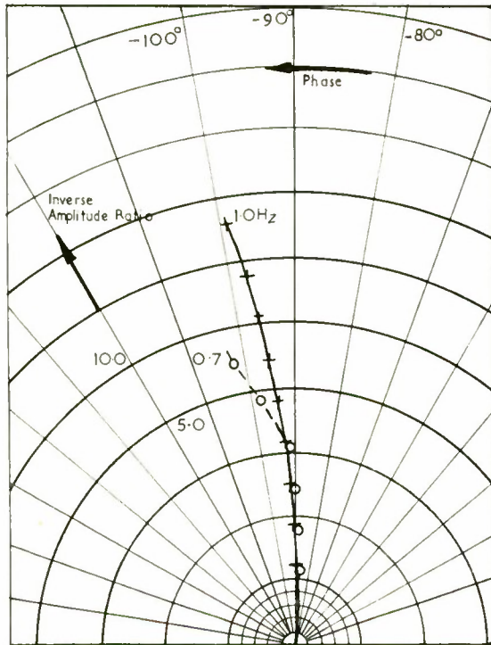
FIG. 18. Inverse Nyquist Plot for a Six-cylinder Diesel Engine with Transfer Function M(j\omega) G(j\omega) . Theoretical curve +++++. Experimental curve oooo. Points plotted at 0.1 Hz intervals.
