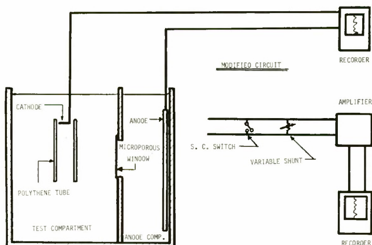
FIG. 1. Schematic sketch of apparatus.
