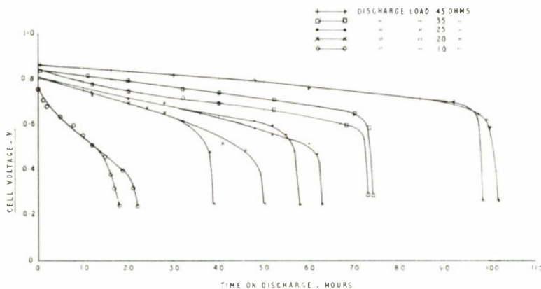
FIG. 6. Discharge Voltage-Time curves for Lead-Silver oxide cells charged for 72 hours at 1.12 V/cell. Effect of discharge load at 20°C.
