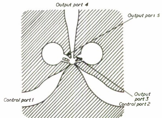
FIG. 4. Fluidic "AND" gate.
