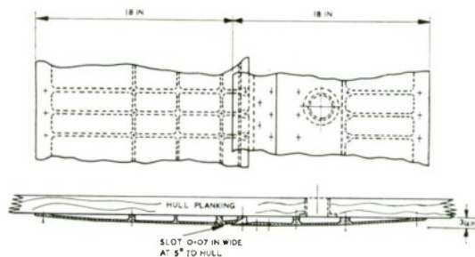
FIG. 2. Details of fairing, duct and ejection slot.
