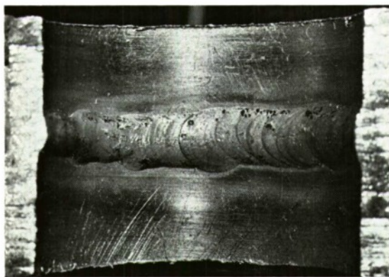
FIG. 3. Moisture 21000 ppm Oxygen <0.1\% \times 5 .
