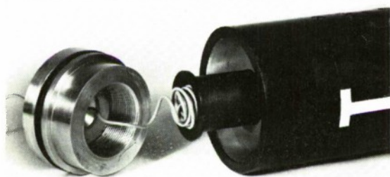
FIG. 8. Trailing Cable Dispenser.
