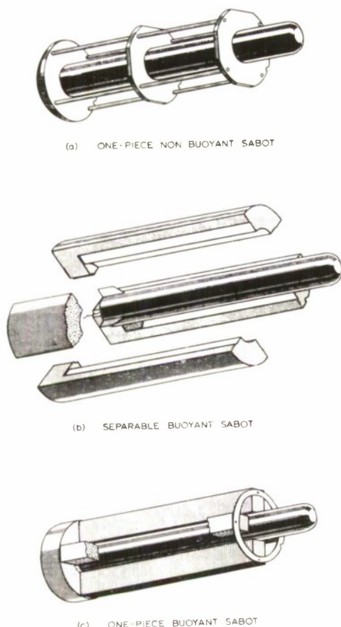
FIG. 4. Sabot Configurations.
