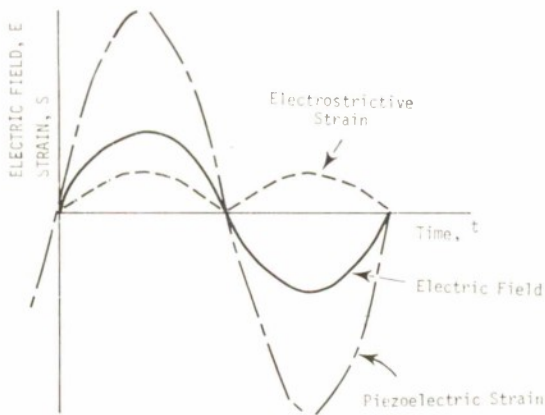
FIG. 1. The variation of strain with electric field for piezoelectric and electrostrictive materials.
