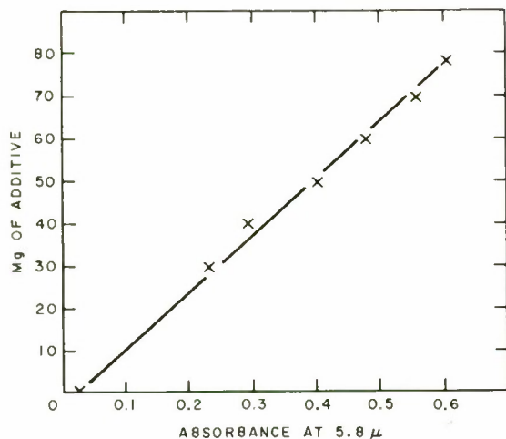
FIG. 7. Calibration graph.
