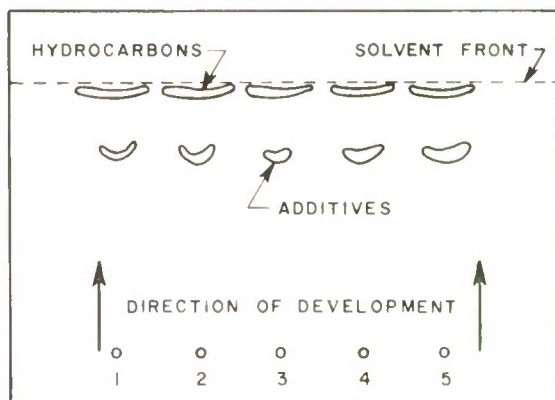
FIG. 3. TLC of turbine oils. Adsorbent: silica gel G. Solvent: CC1 4 .
