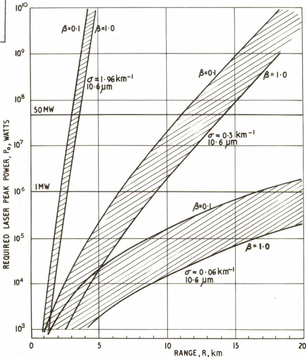
COMPARISON OF REQUIRED LASER POWERS (FOR PbSnTe DETECTOR) FOR A VARIATION OF 10 \times IN BACK SCATTERING CROSS SECTION OF CLOUD.
