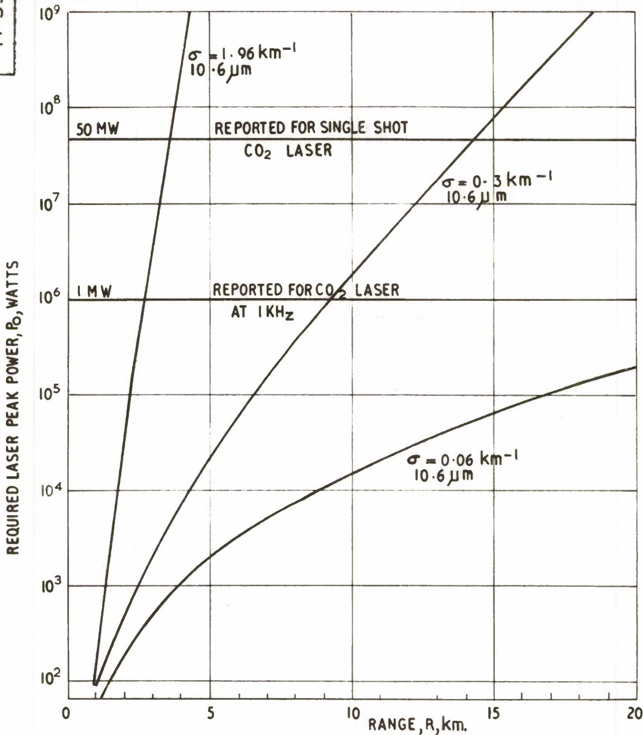
REQUIRED LASER POWER v RANGE FOR DETECTION BY 'CO 2 LIDAR' WITH PbSnTe DETECTOR FOR VARIOUS VALUES OF EXTINCTION COEFFICIENT, σ.
