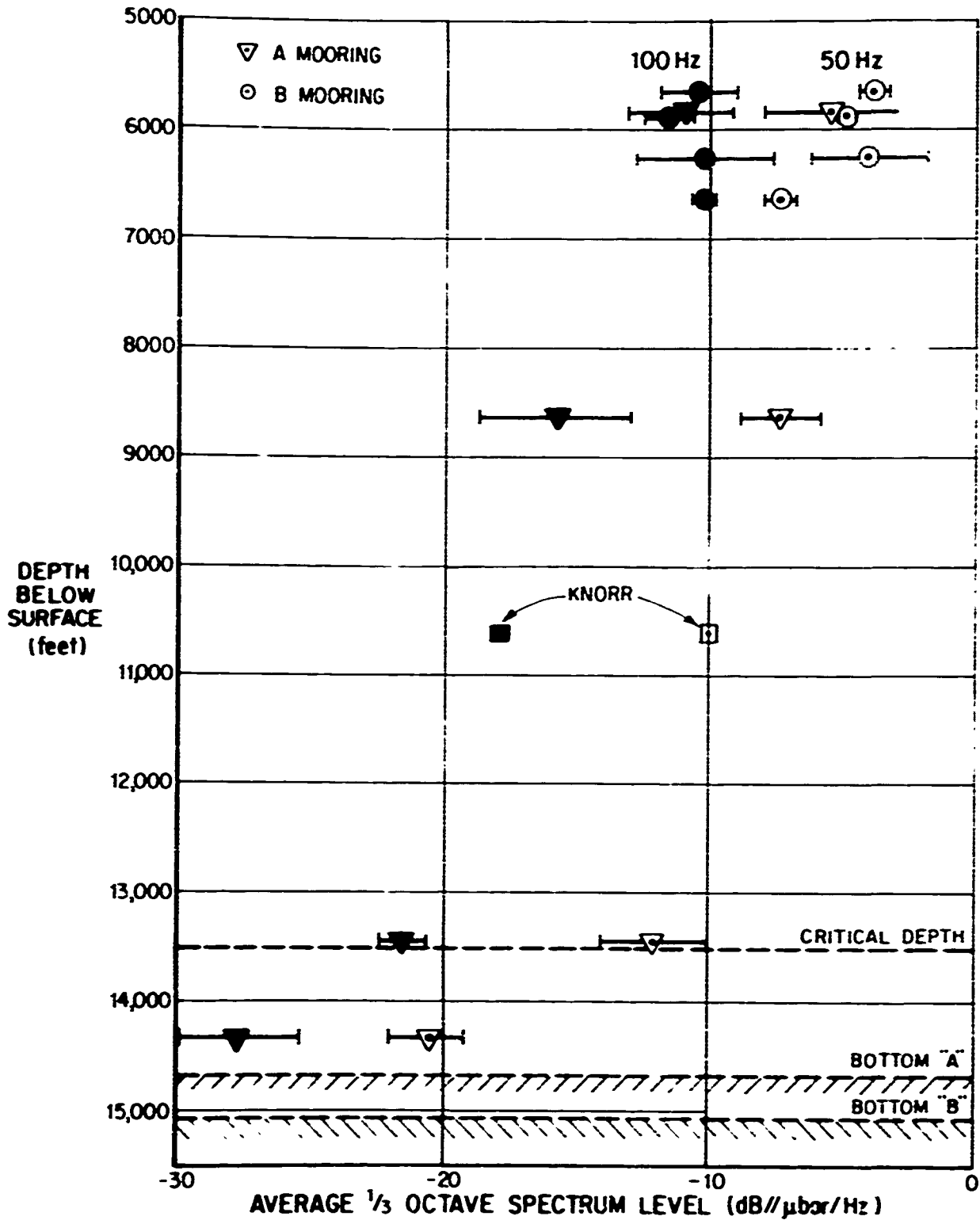
AMBIENT NOISE AVERAGED OVER 15 HALF HOUR INTERVALS DURING A 24 HOUR PERIOD FROM 2000/15-2000/16 (U)
