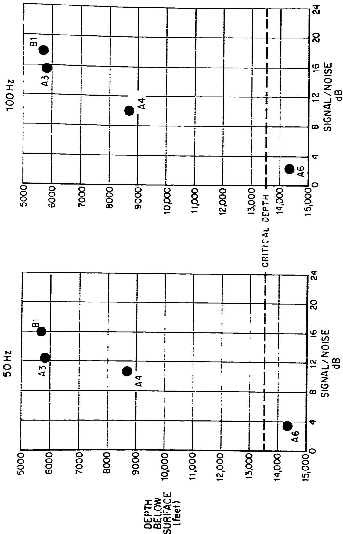
PEAK SHOT SIGNAL TO HOURLY AVERAGE AMBIENT NOISE RATIO VS DEPTH (U)
