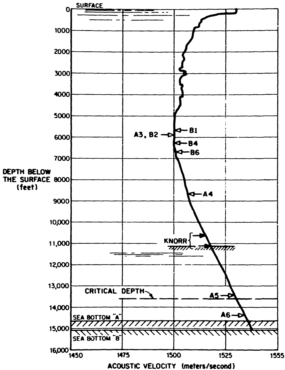
MEASURED 45 NM SE OF ACODAC ARRAYS (U) FIGURE 4
