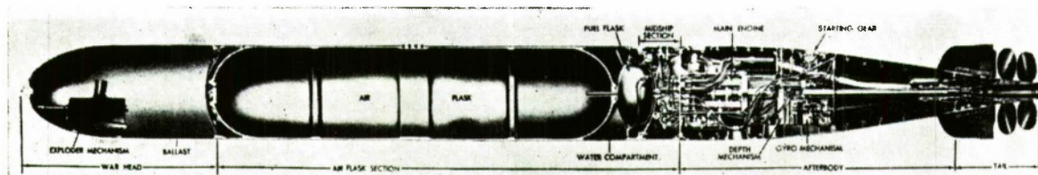
FIG. 37. U.S. Mark 14 weapon.
