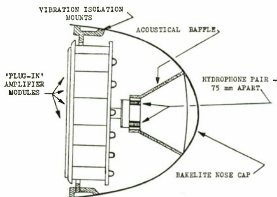
FIG. 33. Homing Head of "PFAU".
