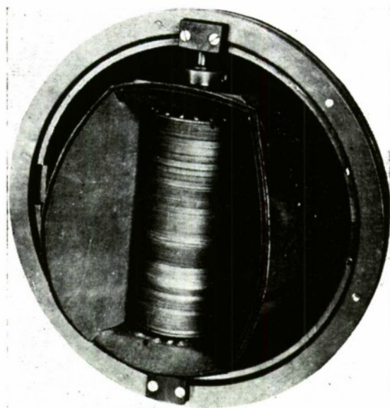
FIG. 34. Scanning Hydrophone from German "LERCHE" Torpedo (1944).
