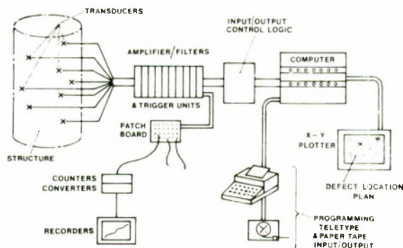
FIG. 6. The AML Defect Location System.
