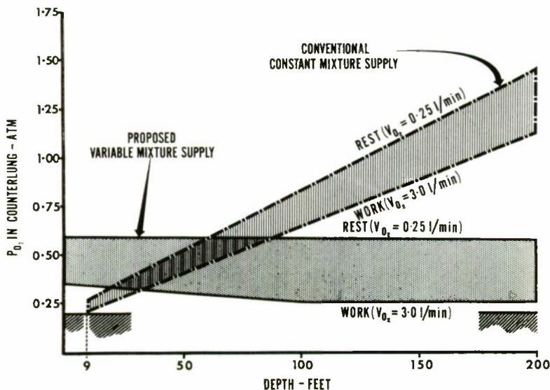
FIG. 3. The relationship of P_{O_2} in the counter lung of semi-closed circuit apparatus to depth. A comparison of a conventional mixture supply system (mass flow 50 l/min. of air) and the proposed variable mixture system (Example 1).
