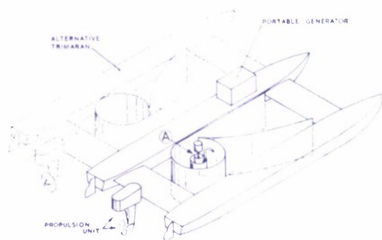
FIG. 3. General layout of prototype skimmer.
