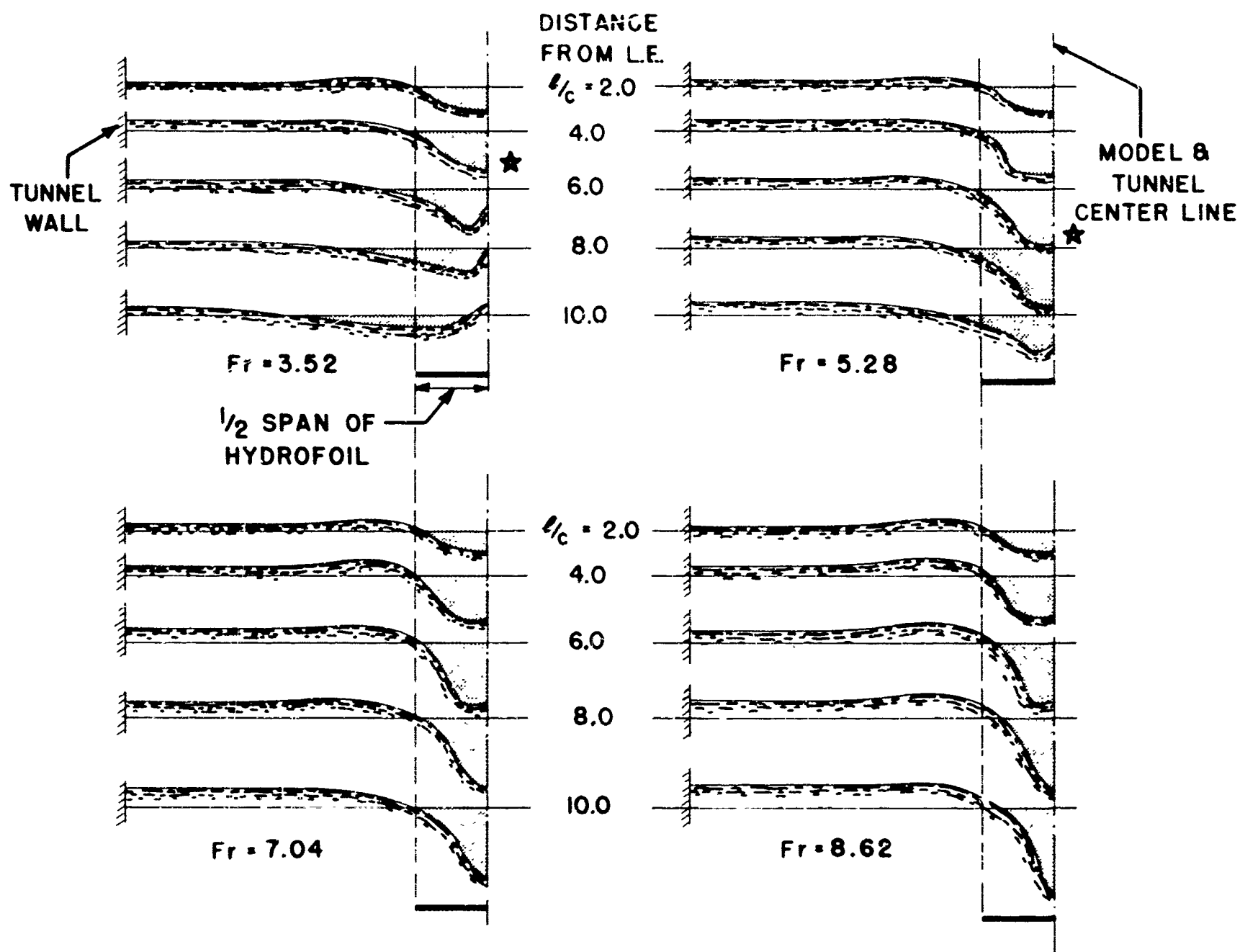
Figure 7. Transverse surface profiles for various Froude numbers at a constant submergence of 0.25 hydrofoil chords and angle of attack of 8^\circ . The "star" on the figure denotes the location of maximum surface depth.
