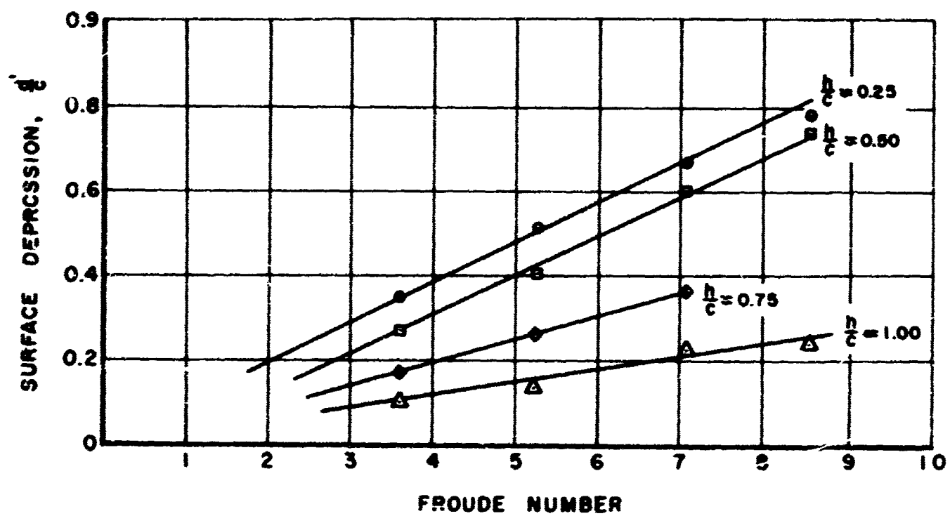
Figure 12. Maximum surface depression as a function of Froude number and submergence ratio.
