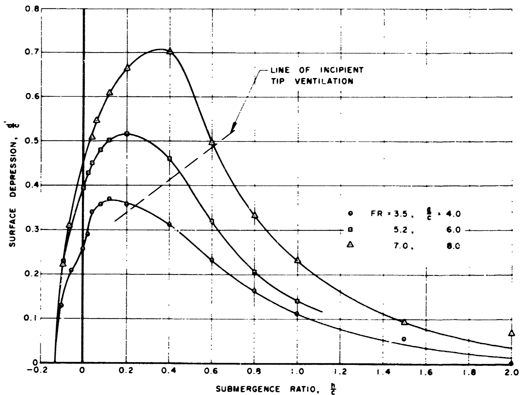
Figure 9. Maximum surface depression behind hydrofoil as a function of submergence and Froude number. The angle of attack is 8^\circ and the aspect ratio of the hydrofoil is 4/3 .
