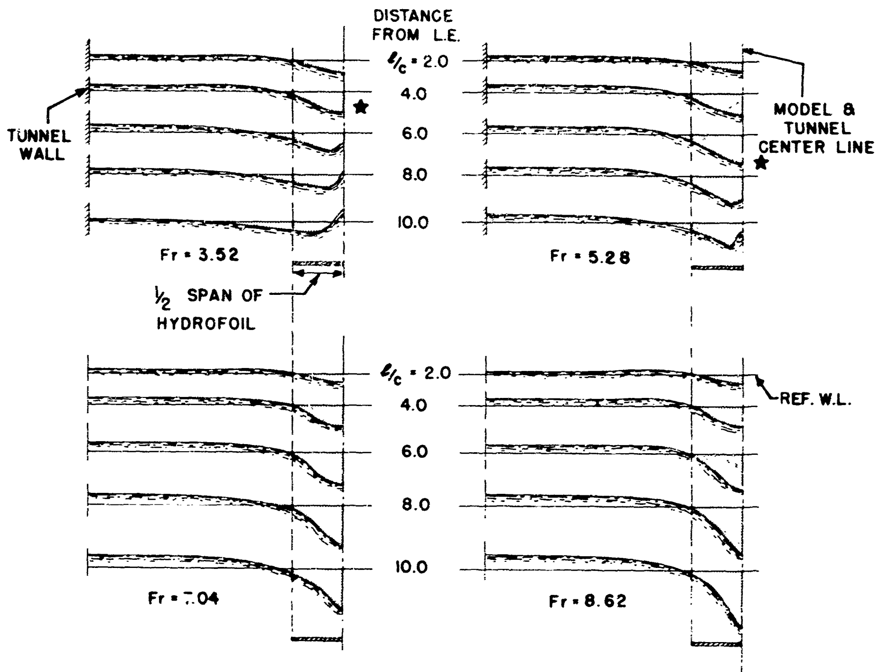
Figure 8. Transverse surface profiles for various Froude numbers at a constant submergence of 0.50 hydrofoil chords at an angle of attack of 8^\circ . The "star" on the figure denotes the location of maximum surface depth.
