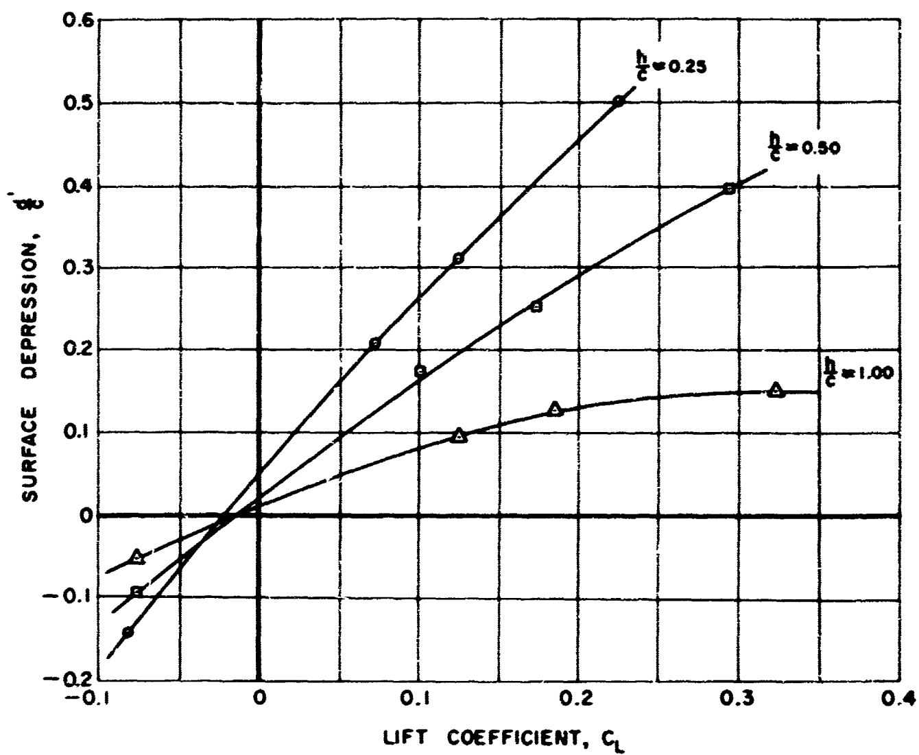
Figure 11. Maximum surface depression as a function of depth and lift coefficient for a Froude number of 5.3 (based on chord). The aspect ratio is 4/3.
