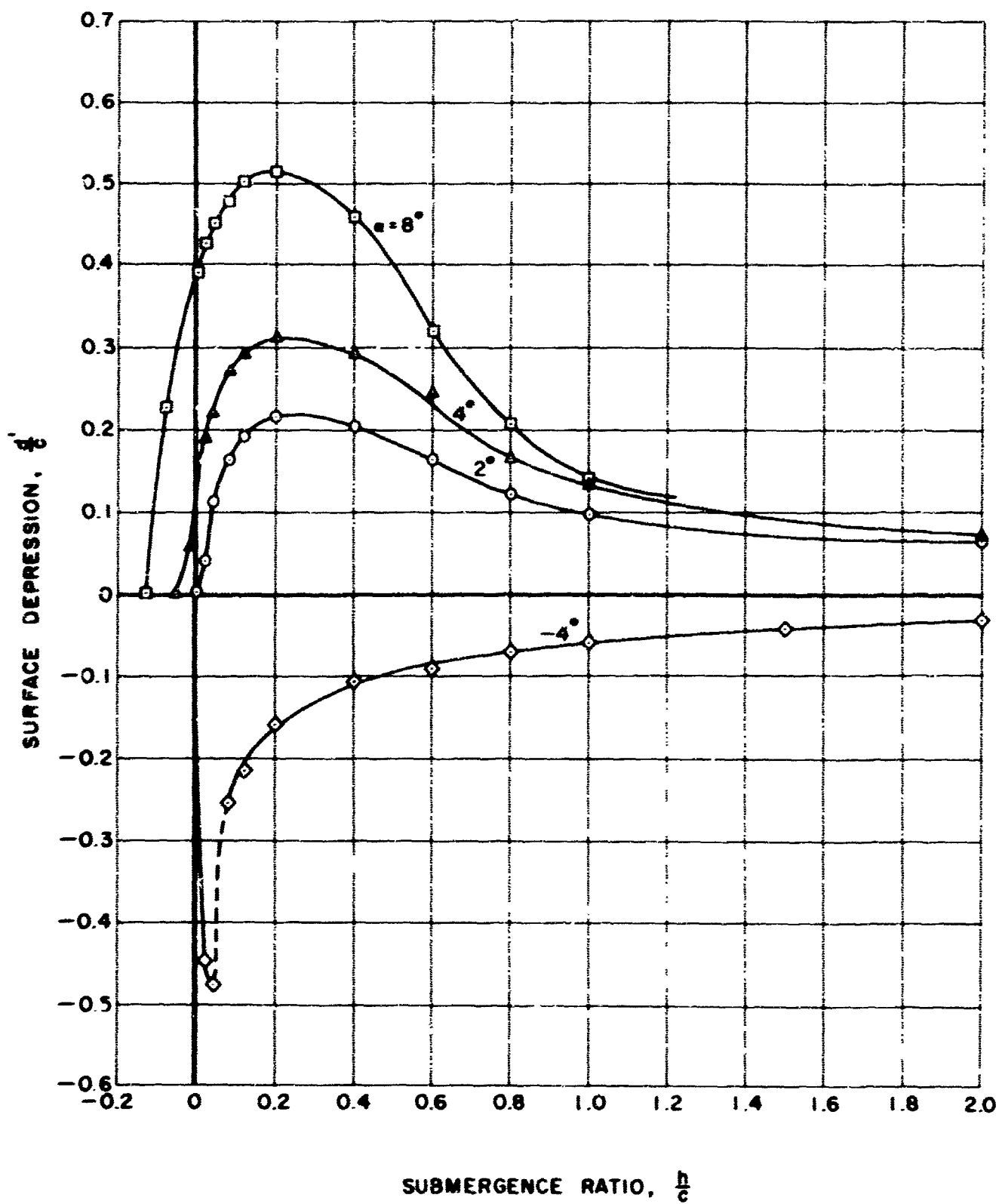
Figure 10. Maximum surface depression behind hydrofoil as a function of submergence ratio and angle of attack. The Froude number is 5.28 (based on chord) for all angles. The aspect ratio of the hydrofoil is 4/3 .
