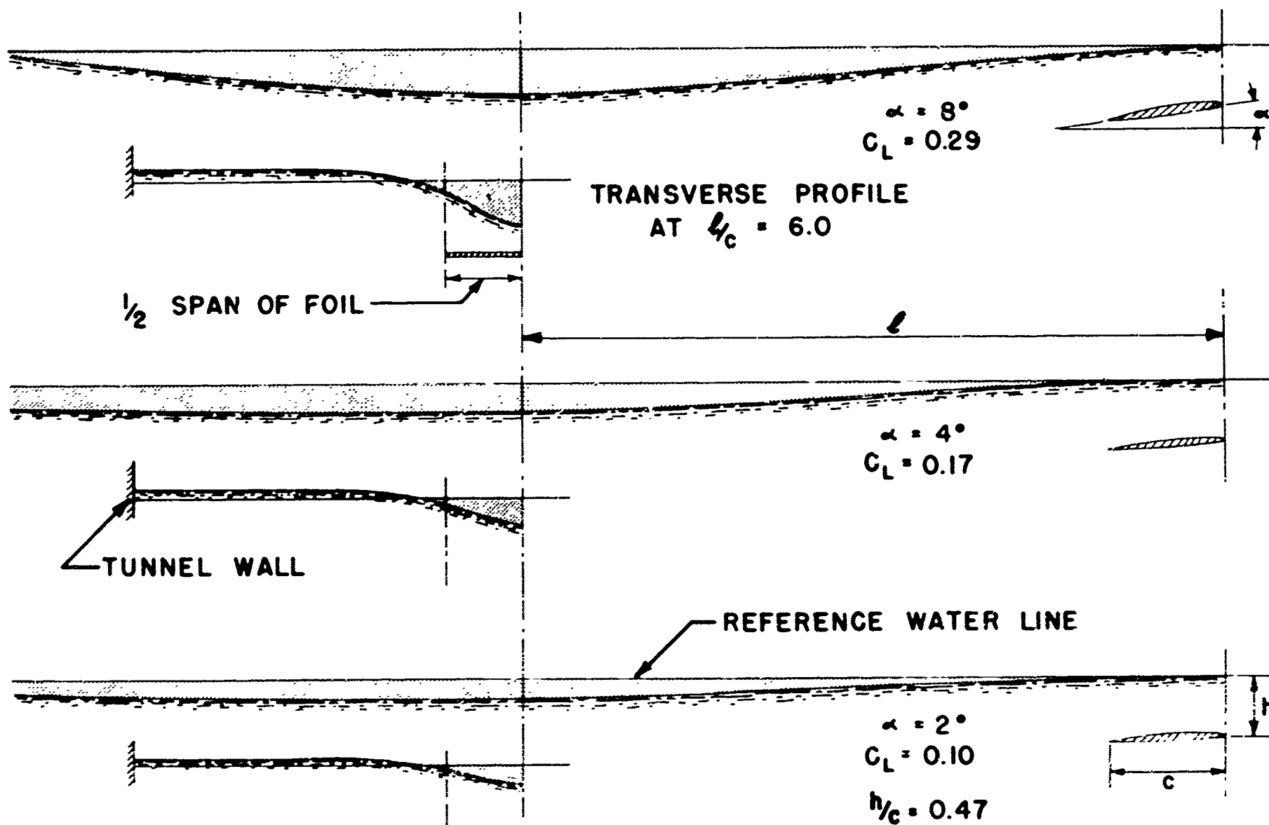
Figure 5. The effect of angle of attack on the water surface profile behind the hydrofoil. The hydrofoil in each case is submerged one-half of its chord length and the Froude number based on chord is 5.3. The aspect ratio of the hydrofoil is 4/3.
