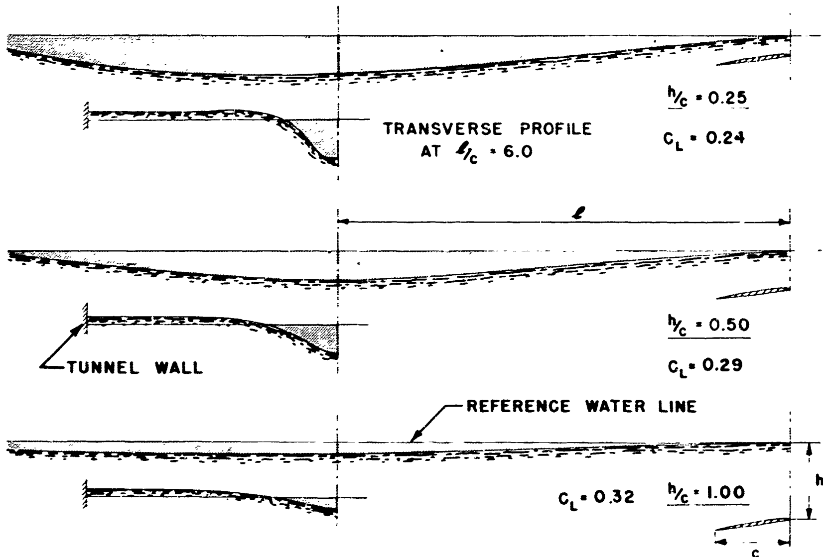
Figure 4. The effect of hydrofoil depth on the water surface profile. The Froude number based on chord is 5.3 and the angle of attack is 8^\circ . For each depth, a longitudinal profile on the centerline of the hydrofoil and a transverse profile six chord lengths downstream are shown. The aspect ratio of the hydrofoil is 4/3 .
