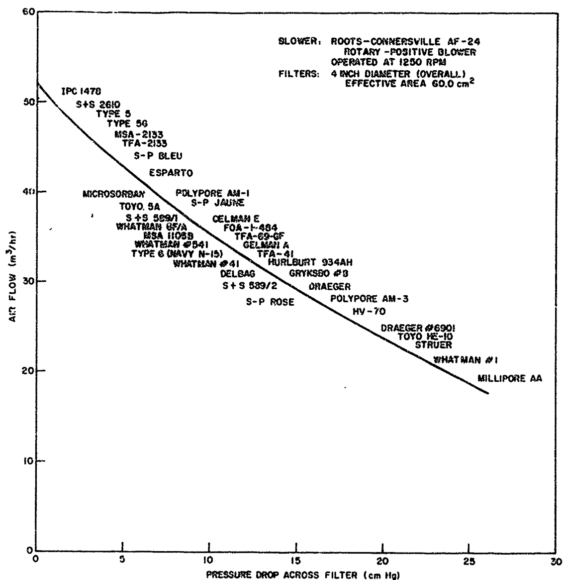
Fig. 1 — Pressure-flow characteristics of filter materials in a positive-displacement blower system.
