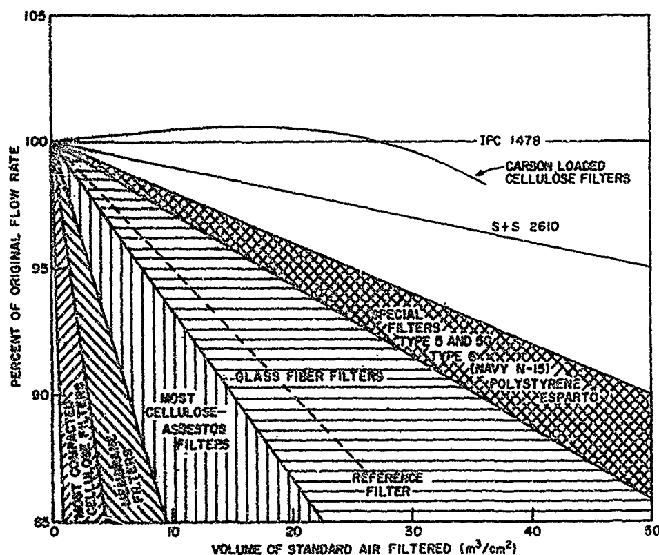
Fig. 2 — Relative clogging rates of various classes of air-filter materials
