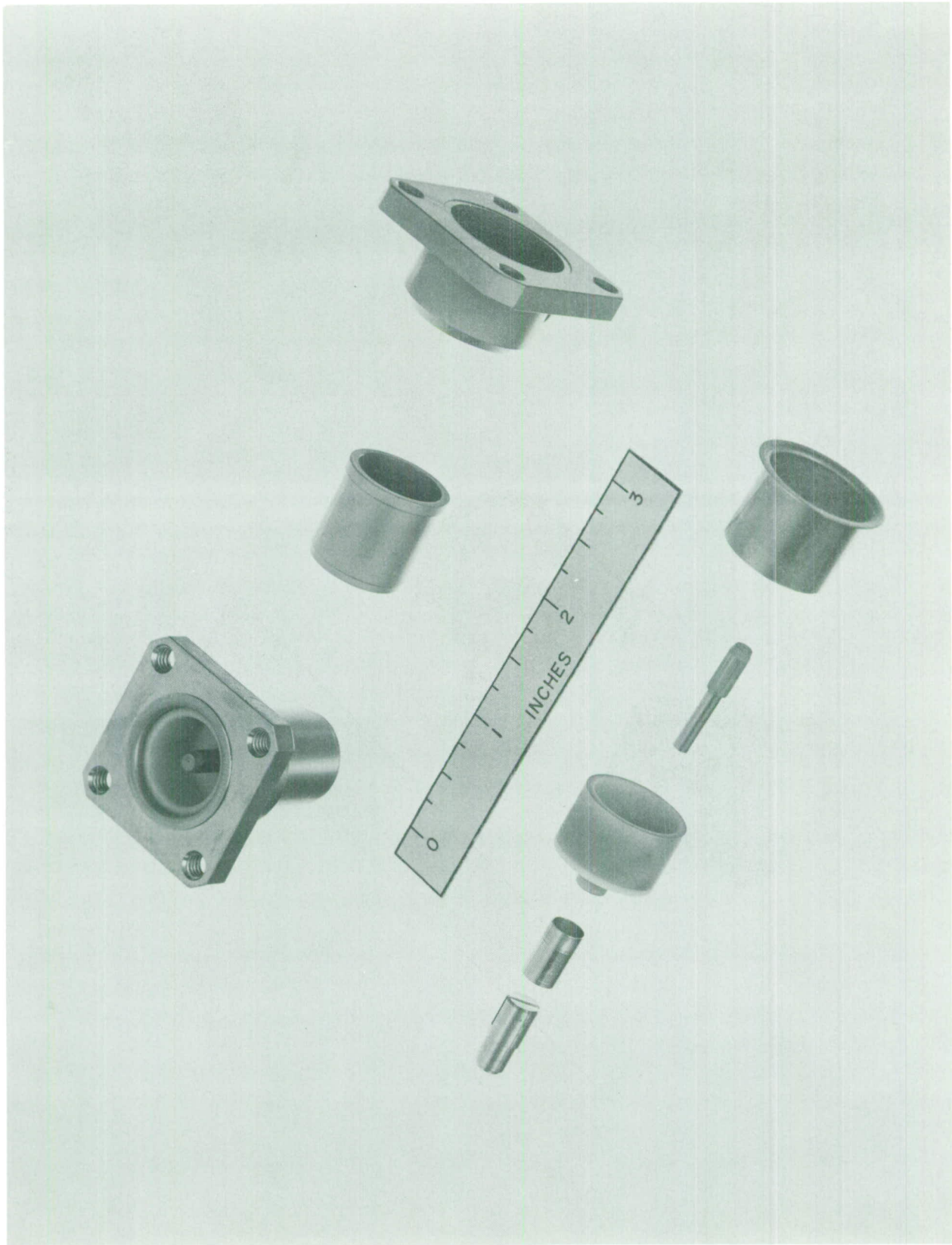
Fig. 14 - A complete rf window assembly and an exploded view of the component parts. This window was used in the grounded circuit tube.
