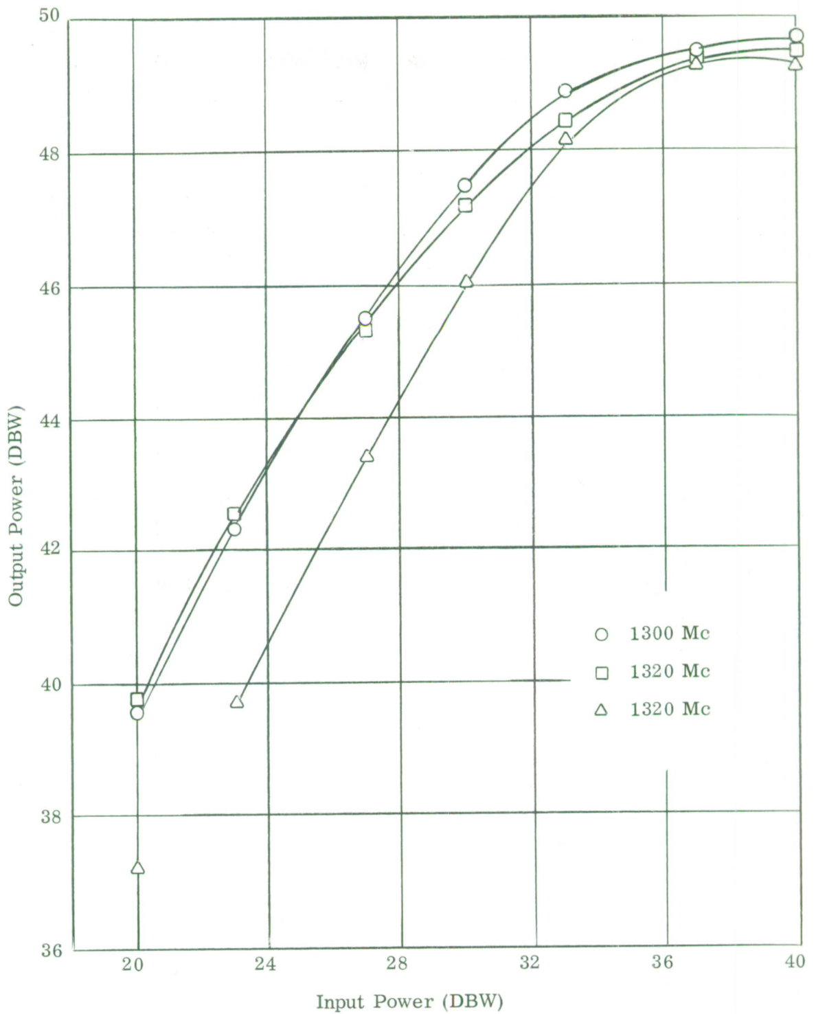
Fig. 42 - Output power vs input power as measured on the ceramic barrel grounded cathode tube shown in Fig. 41. Table III lists the operating parameters of the tube during these measurements.
