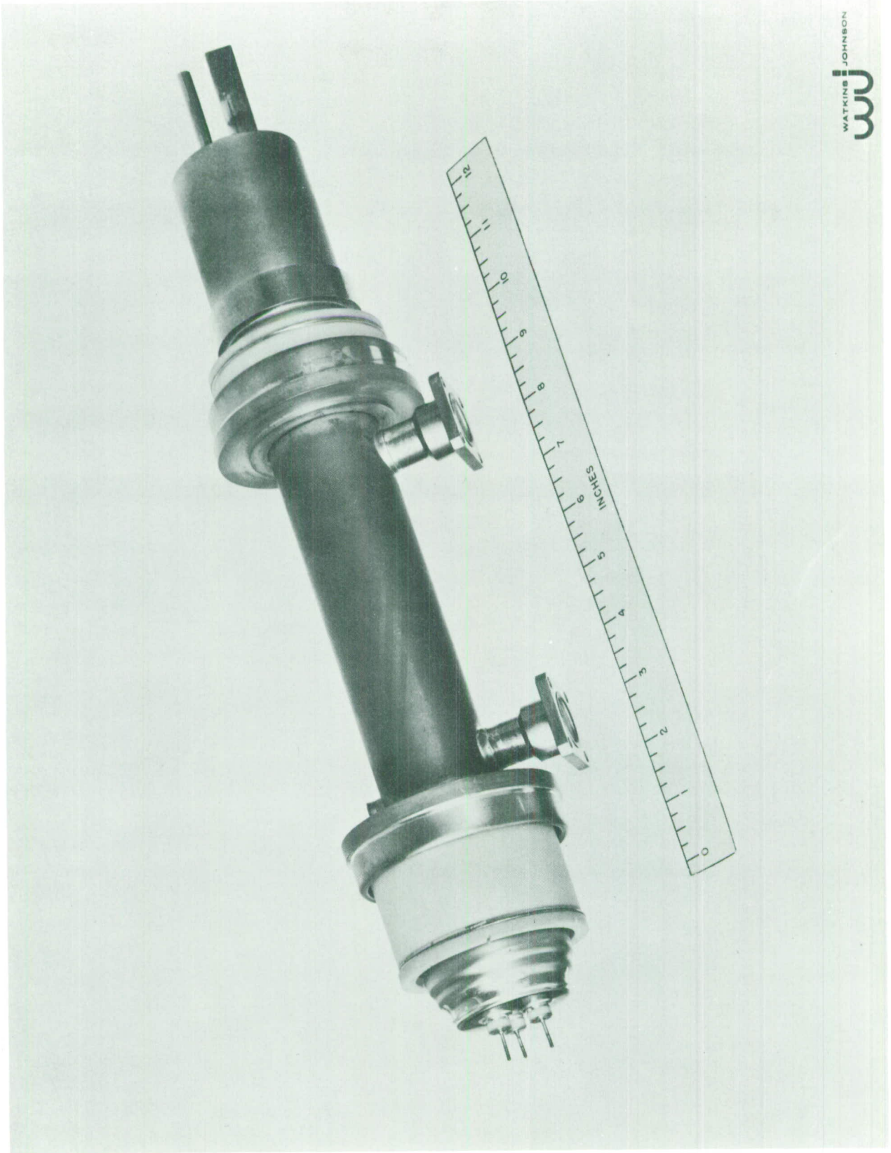
Fig. 18 - The first tube constructed was the grounded circuit tube shown above. Beam efficiency of over 30 percent was measured on this tube.
