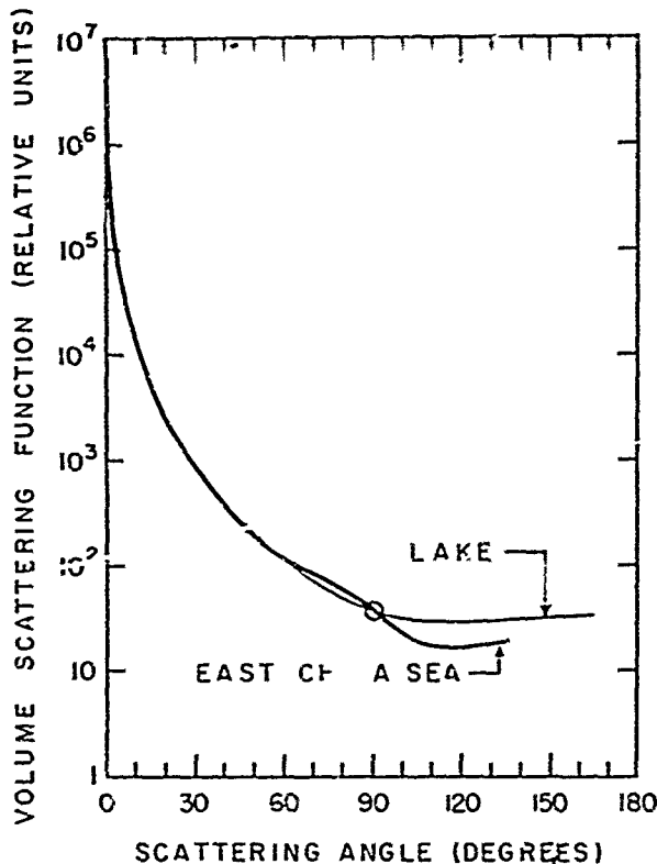
FIG. 10. Comparison of the shape of the in situ volume scattering function data for Lake Winnepesaukee, New Hampshire, from Fig. 9 with the shape of a curve representing the in vivo scattering data obtained by Koslyaninov (see reference 15) using a shipboard laboratory apparatus and a sample of water taken from the East China Sea. The curves have been normalized at a scattering angle of 90° (circled point) for purposes of shape comparison. Koslyaninov used blue light isolated by means of an absorption filter having an effective wavelength of 494 m \mu ; he reported data at scattering angles of 1, 2.5, 4, 6, 10, 15, 30, 50, 70, 110, and 144 deg. The curves are similar in shape for scattering angles less than 60°
