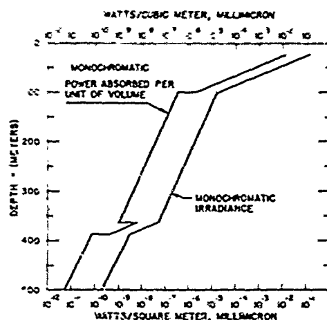
FIG. 32. Superimposed semilogarithmic plots of monochromatic downwelling irradiance vs depth and monochromatic radiant power absorbed per unit of volume vs depth illustrate the (approximate) relation between these quantities expressed by Eq. (20). Monochromatic downwelling irradiance is the total monochromatic radiant power per unit of area received by the upper surface of a horizontal plane at arbitrary depth z . The product of this irradiance and its depth attenuation function (slope of its depth profile) is, within about 2%, equal to the monochromatic power absorbed per unit of volume. Thus, at a depth of 50 m in Fig. 32, H(50, -) = 6.3 \times 10^{-3} \text{ W/(m}^2, \text{m}\mu) , K(50, -) = 0.114 \text{ ln/m} , and dP(50)/dz \approx (6.3 \times 10^{-3})(0.114) = 7.2 \times 10^{-4} \text{ W/(m}^3, \text{m}\mu) . Neither of the curves in this figure represent specific experimental data, but the irradiance profile is typical of the Pacific Ocean off California. The presence of a deep scattering layer is shown below 350 m.
