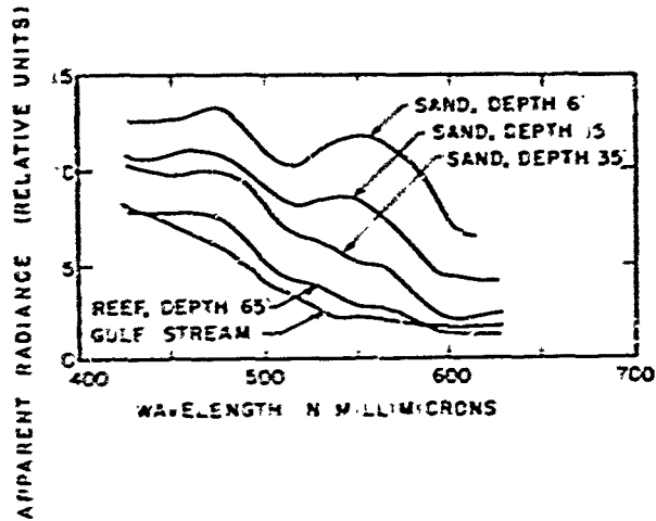
FIG. 2. Spectroradiometric curves of light from the nadir reaching a spectrograph in an airplane 4300 ft above the same ocean locations as in Fig. 1. Spectral resolution: 7.0 m \mu ; spatial resolution: 3.2 \times 10^{-4} sr.
