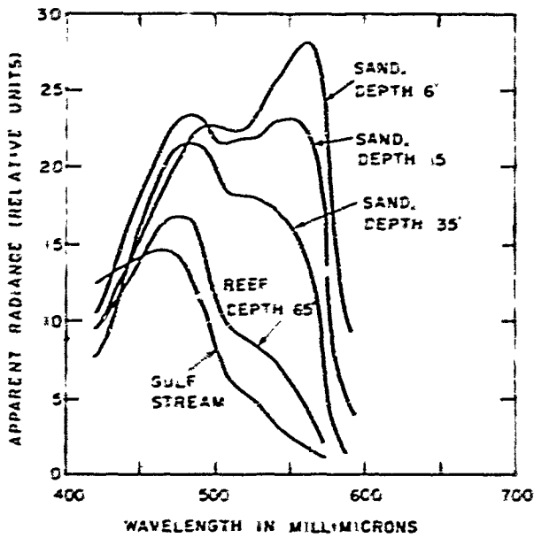
FIG. 1. Spectroradiometric curves of light from the nadir reaching a spectrograph mounted in a glass-bottomed boat over shoals off Dania, Florida (March 1944). Spectral resolution: 7.7 m \mu ; spatial resolution: 2.0 \times 10^{-4} sr.
