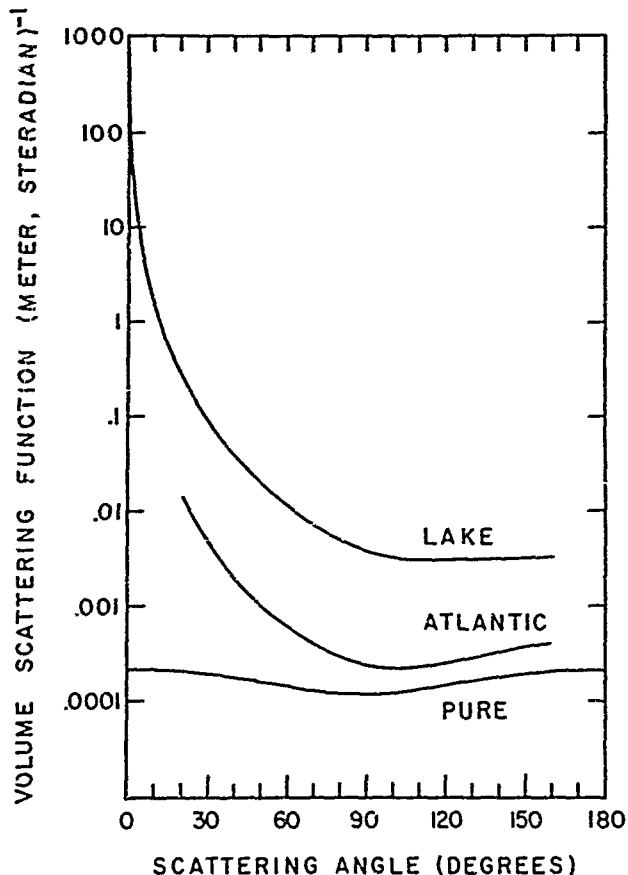
FIG. 9. Volume scattering function curves for pure water (Dawson and Hulbert, see reference 12), the Atlantic between Madeira and Gibraltar (Jerlov, see reference 8), and the Diamond Island Field Station, Lake Winnepesaukee, New Hampshire. The upper curve (lake) represents in situ measurements at 5° intervals between scattering angles 20° > \theta > 160° by means of a conventional type, pivoted-arm scattering meter and a single datum at \theta = 0.5^\circ obtained in situ with the coaxial scattering meter shown schematically in Fig. 8; the data are of 20 August 1961; and are for green light isolated by means of a Wratten No. 61 filter
