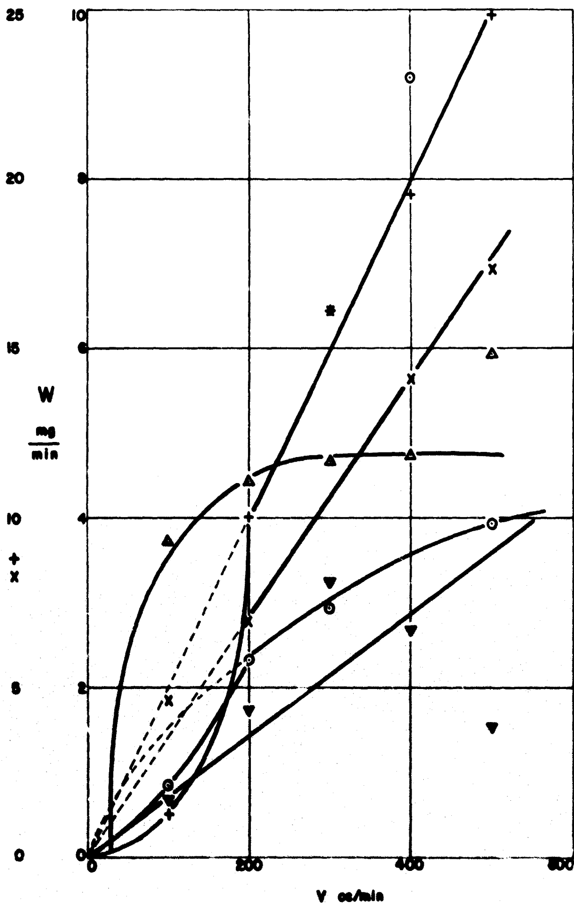
Figure 9. Total weight of deposits in 1 min W = W_1 + W_2 as a function of flow rate v . Saccharin, \times Saccharin + 1% Cab-O-Sil, Carbowax 6000, \Delta Cab-O-Sil, + Carbowax 6000 + 1% Cab-O-Sil.
