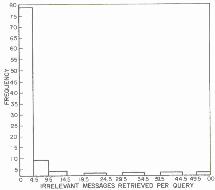
Fig. 7. Frequency of Occurrence of Irrelevant Messages Retrieved — All Queries, No Expansion
