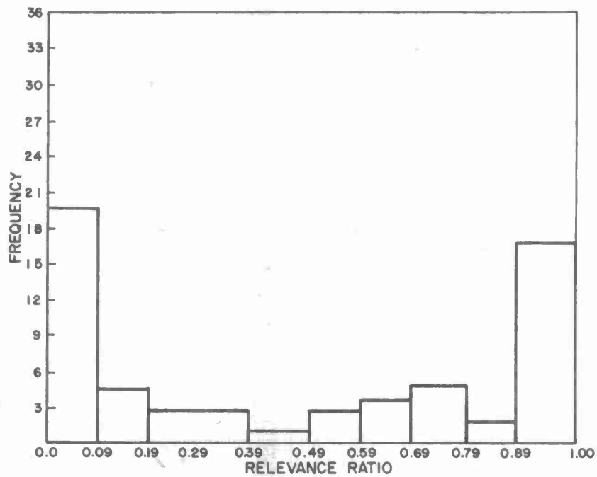
Fig. 4. Frequency of Occurrence of Relevant Messages Retrieved — Multiple Factor Queries, Synonym Expansion (R ≠ 0)
