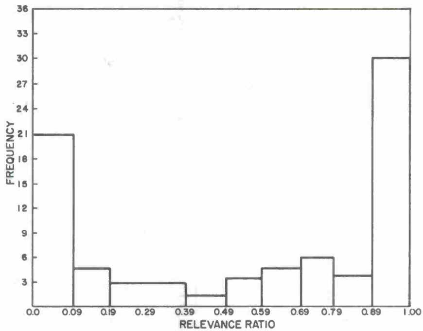
Fig. 3. Frequency of Occurrence of Relevant Messages Retrieved — All Queries, Synonym Expansion (R ≠ 0)
