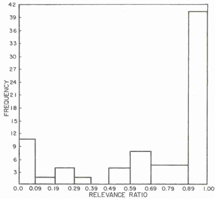
Fig. 5. Frequency of Occurrence of Relevant Messages Retrieved — All Queries, Complete Expansion (R ≠ 0)
