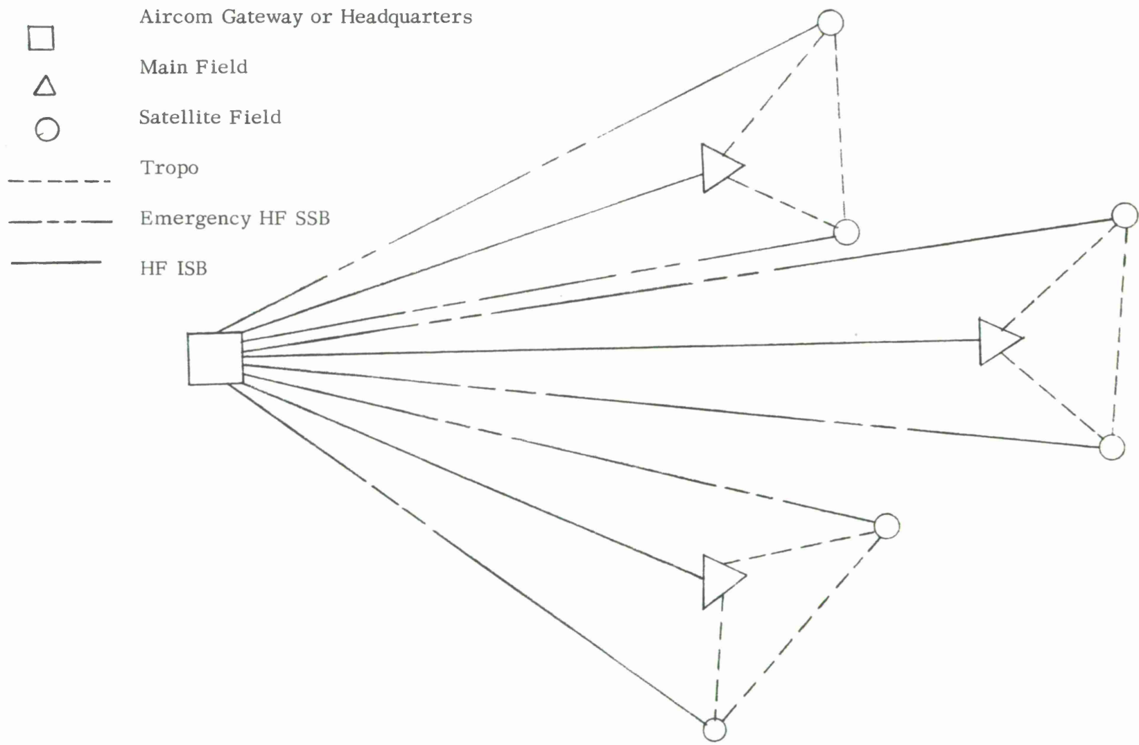
Figure 2. Recommended Alternate Routing System
