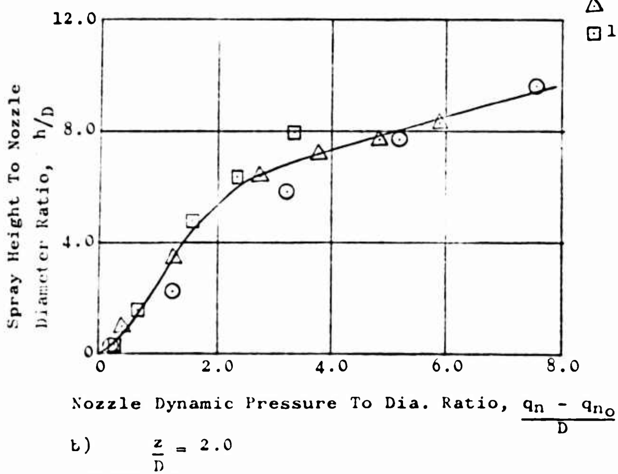
FIG. 9 SPRAY HEIGHTS AT VARIOUS NOZZLE PRESSURES
