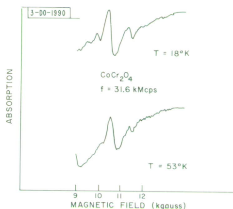
Fig. V-2. The spin resonance spectrum in the "uniform mode" of \text{CoCr}_2\text{O}_4 as a function of magnetic field at 18^\circ and 53^\circ\text{K} .
