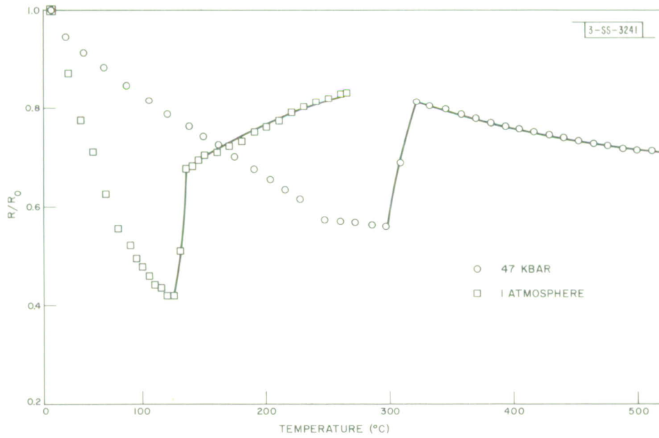
Fig. III-6. Relative resistance ( R/R_0 ) vs temperature for \text{Ag}_2\text{Se} at atmospheric pressure and at 47 kbar. At atmospheric pressure, resistivity in ohm-cm is equal to (1.02 \times 10^{-3}) (R/R_0) .
