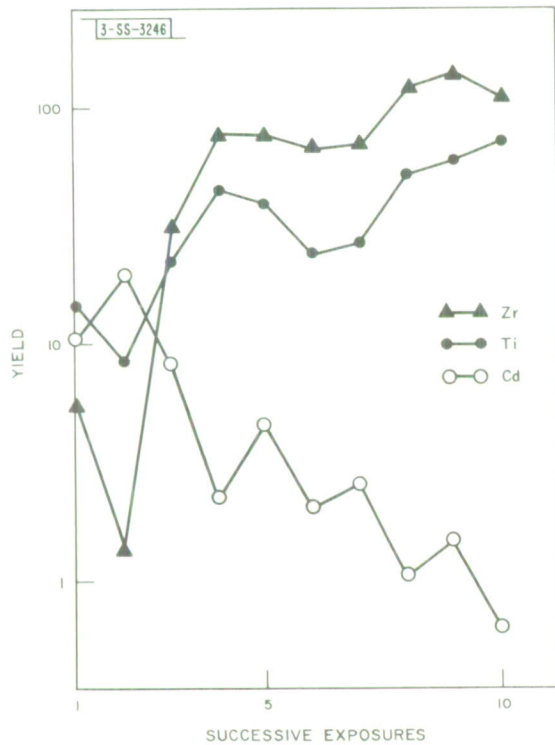
Fig. III-13. Mass spectrographic analysis of mixed CdO , TiO_2 , and ZrO_2 . Yields of cadmium, titanium, and zirconium ions in successive equal exposures.
