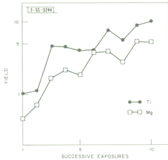
Fig. III-11. Mass spectrographic analysis of powdered MgTiO_3 . Yields of magnesium and titanium ions in successive equal exposures.
