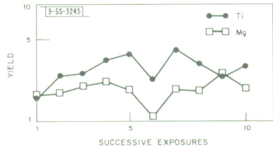
Fig. III-12. Mass spectrographic analysis of mixed MgO and TiO_2 powders. Yields of magnesium and titanium ions in successive equal exposures.
