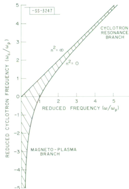
Fig. IV-2. Poles and zeros of the dielectric constant for propagation parallel to the magnetic field.
