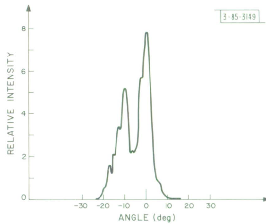
Fig. I-4. Radiation pattern in junction plane of InAs laser at six times the threshold current. Laser was operated at 4.2°K.
