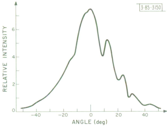
Fig. 1-5. Radiation pattern in a plane perpendicular to junction plane of InAs laser operated at 4.2°K.
