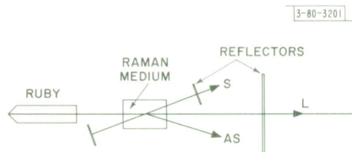
Fig. II-2. Experimental arrangement for obtaining off-axis stimulated Raman emission.
