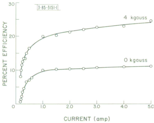
Fig. 1-7. Effect of magnetic field on external efficiency of InAs laser at 4.2°K.
