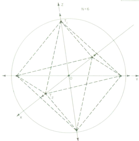
Fig. 8. Geometry showing the chosen pointing directions for 6 antennas .
