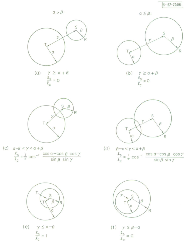
Fig. 3. Various situations that may exist for the relative values of the angles a , \beta , and \gamma . The value \ell_s/\ell_c is given in each case.
