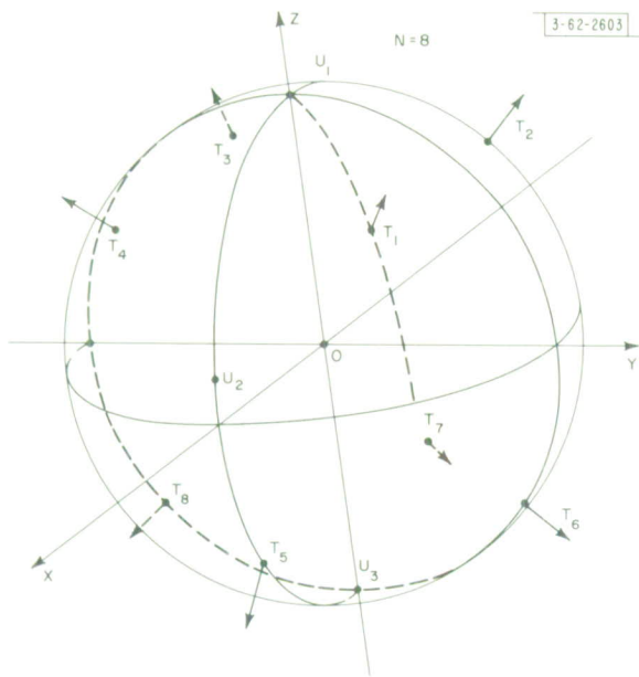
Fig. 10. Geometry showing the chosen pointing directions for 8 antennas.
