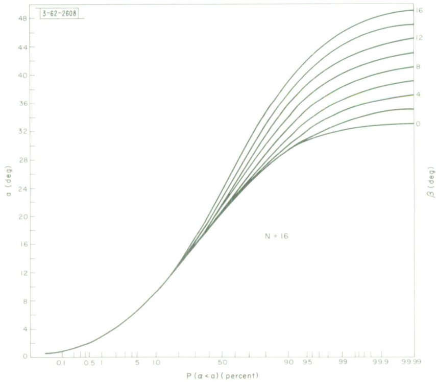
Fig. 15. Probability that receiver is at an angle less than \alpha from the pointing direction of the antenna in operation for the 16-antenna geometry (Fig. 14).
