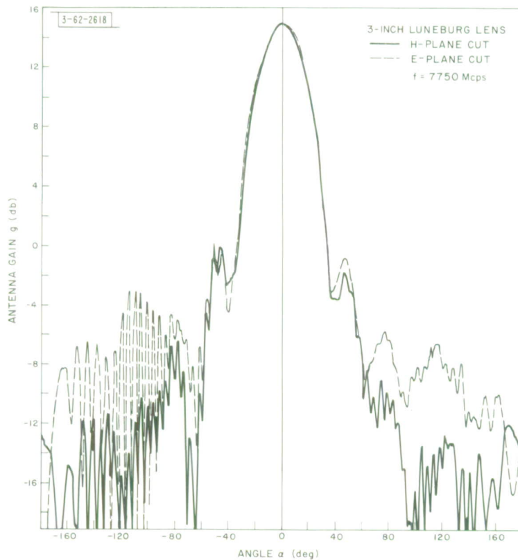
Fig. 25. Pattern of a circular pipe of 1-inch aperture butted against a Luneburg lens of 3-inch diameter taken at a frequency of 7750 Mcps.
