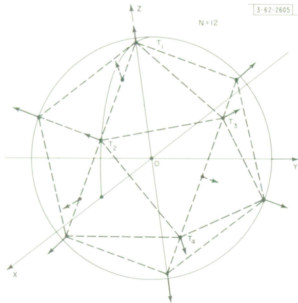
Fig. 12. Geometry showing the chosen pointing directions for 12 antennas.
