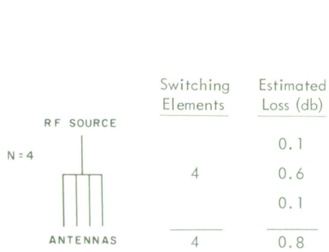
(a) 4-antenna system.
