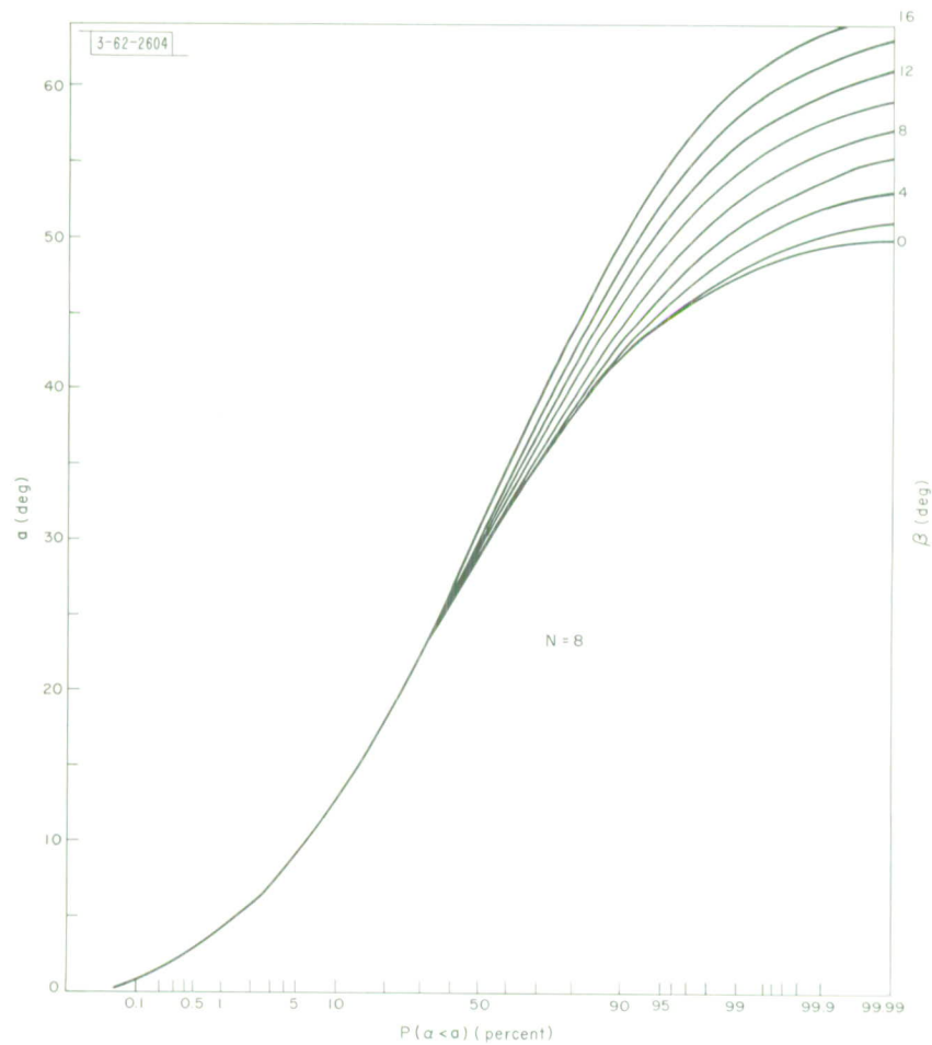
Fig. 11. Probability that receiver is at an angle less than \alpha from the pointing direction of the antenna in operation for the 8-antenna geometry (Fig. 10).
