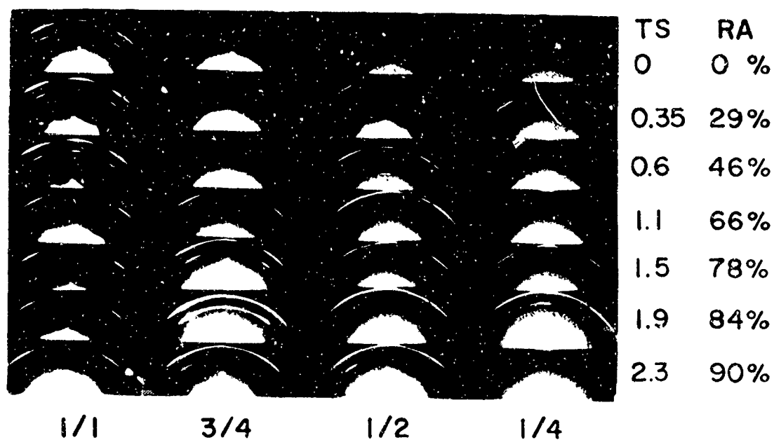
Fig. 5 IIO diffraction ring composite, swaged Cb-450, [110] initial texture
