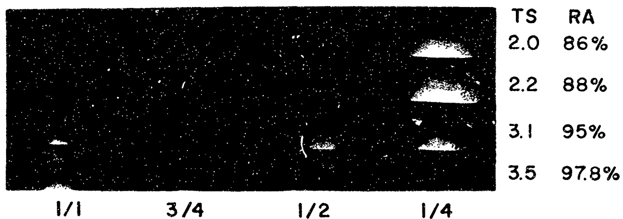
Fig. 4 IIO diffraction ring composite of Cb-150, recrystallized after drawing from random initial texture
