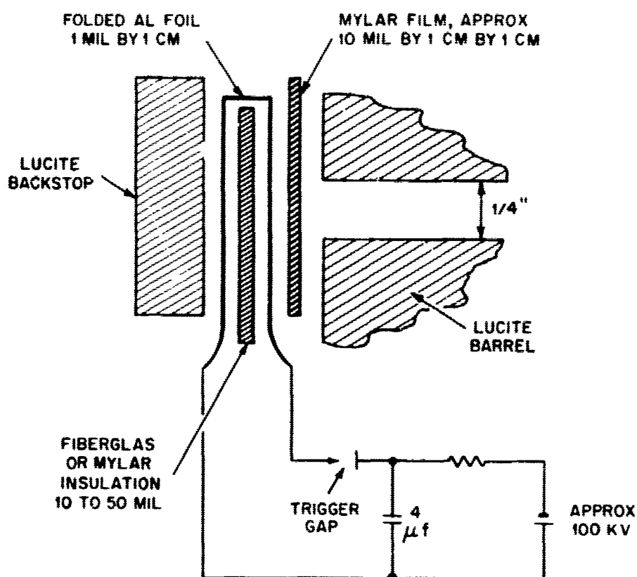
Figure 2. Exploded Diagram of Present Hypervelocity System
