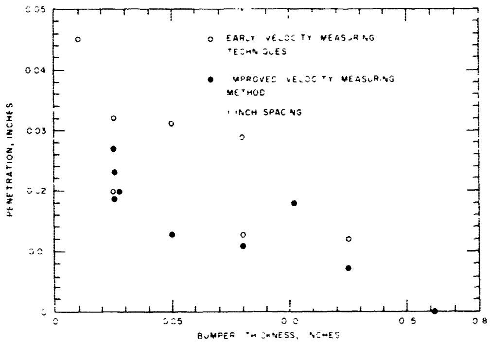
Figure 17. Comparison of Early Data with That Obtained Using the Improved Velocity Measuring Equipment
