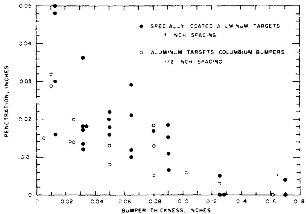
Figure 18. Plot of Maximum Depth of Penetration as a Function of Bumper Thickness for Special Targets and Bumpers
