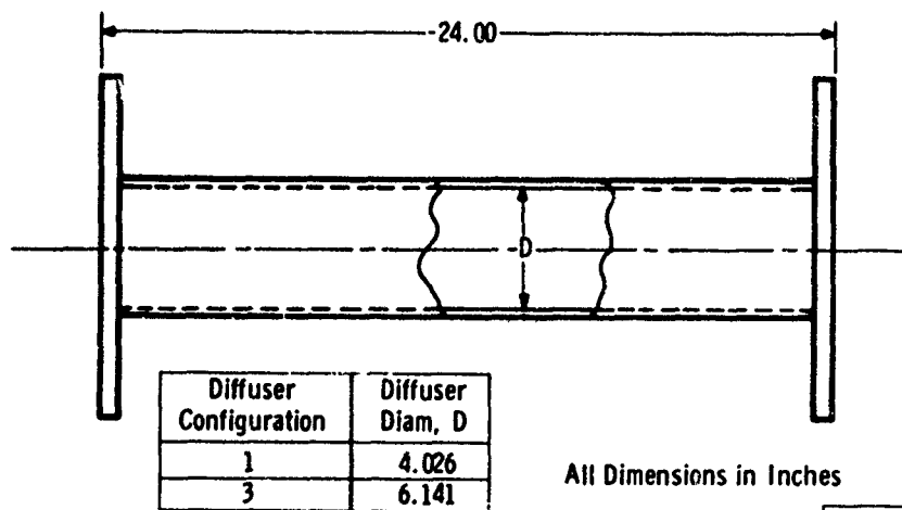
a. Straight Cylindrical Diffuser Configurations 1 and 3
