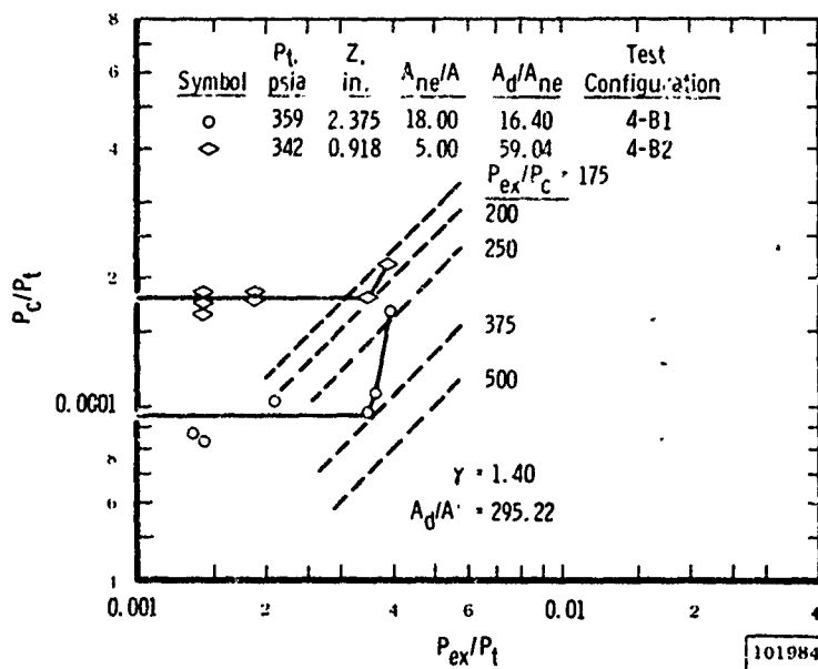
b. Configurations 4-B1 and 4-B2
