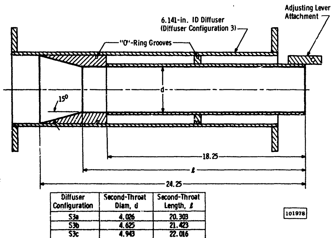
b. Second-Throat Diffuser Configuration S3
