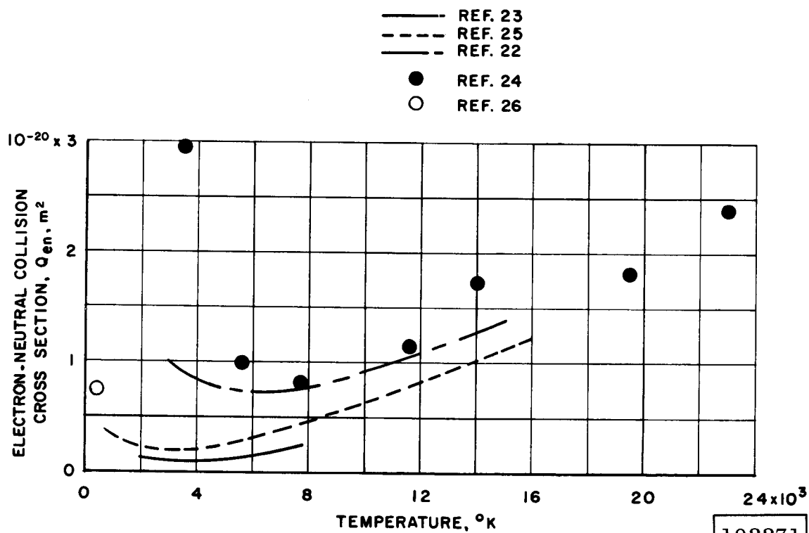
Fig. 2 Electron-Neutral Collision Cross Section for Argon
