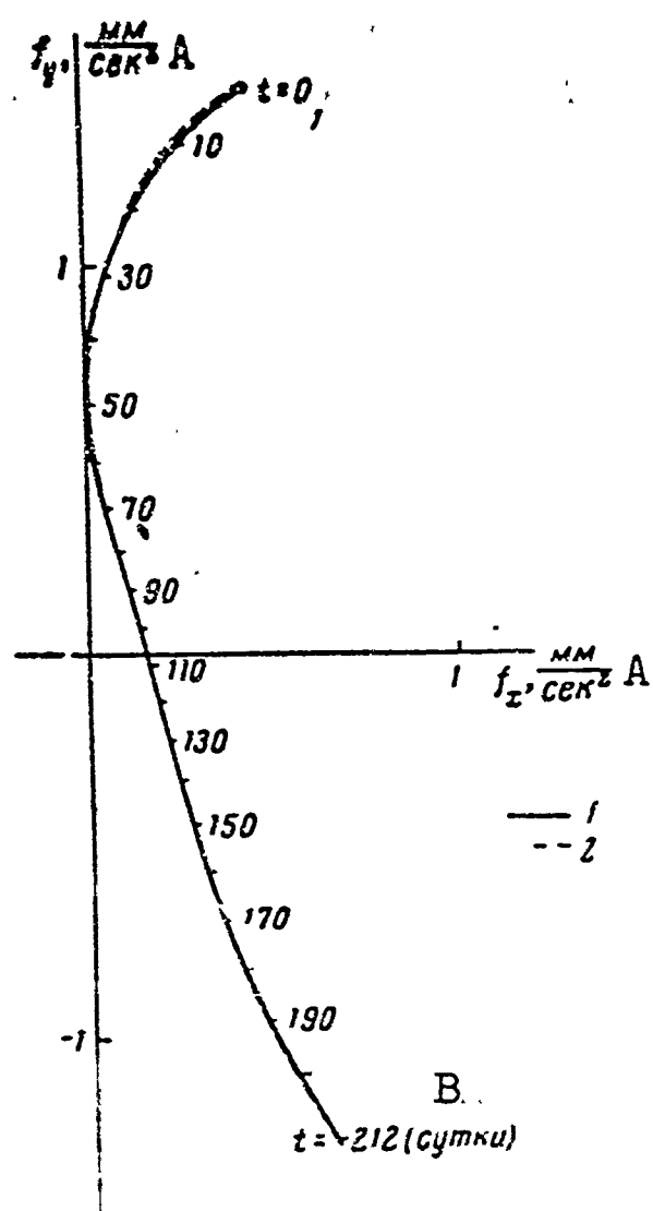
Fig. 7. Variation of magnitude and direction of reactive acceleration. 1) Exact calculation; 2) approximate calculation. A) \text{mm/sec}^2 ; B) days.
