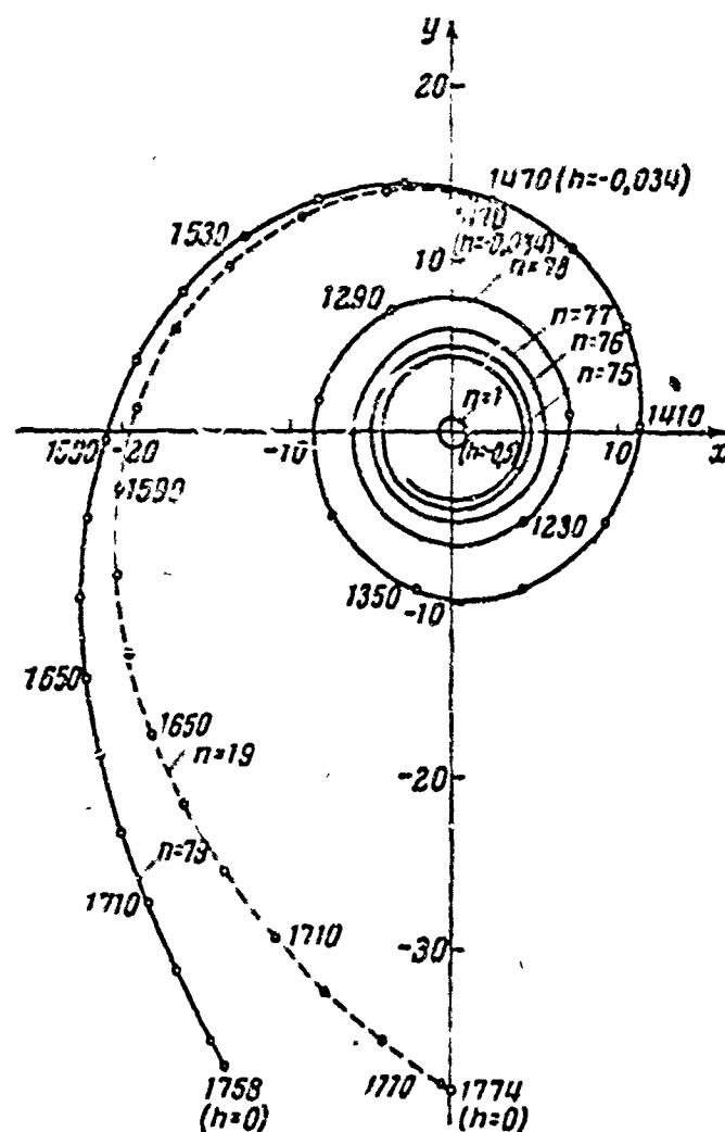
Fig. 4. Example of acceleration trajectory departing from an initially circular orbit (in dimensionless variables). Solid line — trajectory at constant tangential acceleration f = 0.0005 . Dashed line — trajectory
