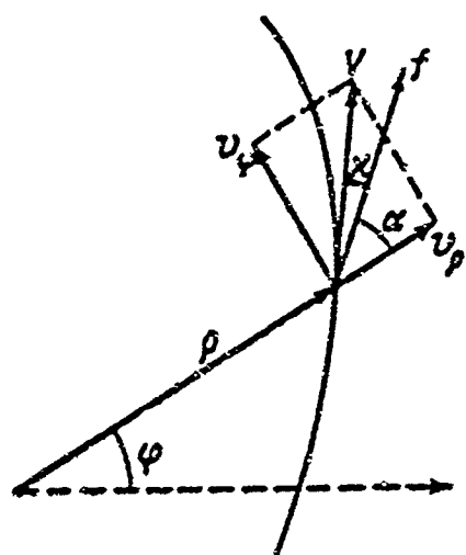
Fig. 1. Coordinate system and mutual position of velocity and thrust-acceleration vectors.
