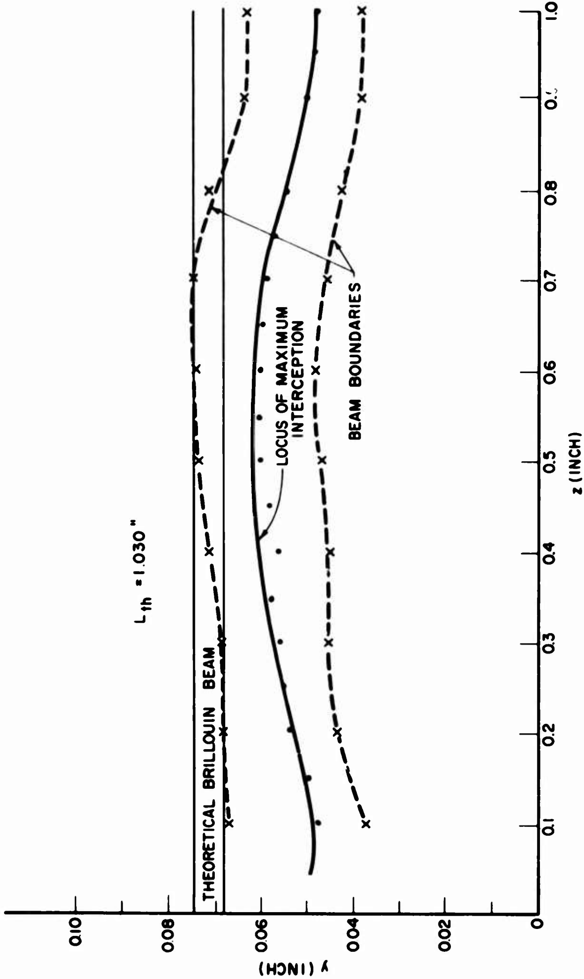
FIG. 7.21 EXPERIMENTAL BEAM CONFIGURATION IN THE INTERACTION REGION.
