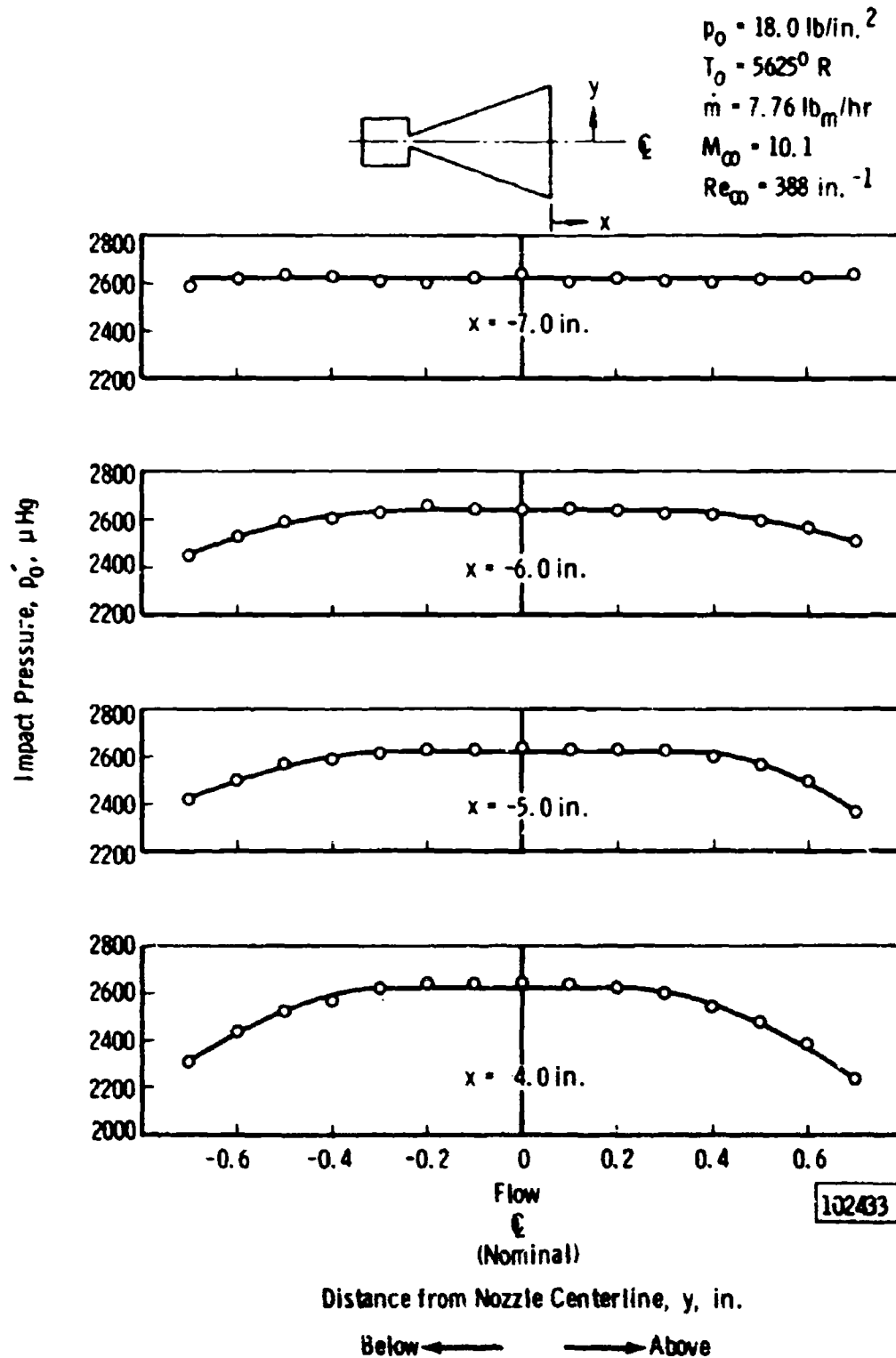
Fig. 5 Radial Impact Pressure Surveys of Nozzle
