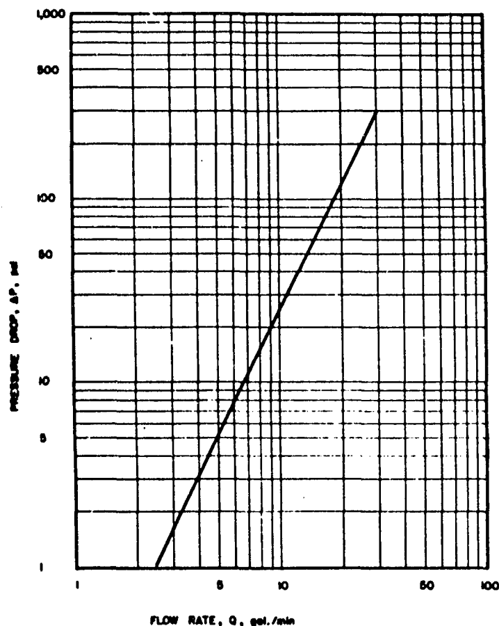
Fig. 9 Typical Pressure Drop Versus Flow Rate Curve for Conical Section
