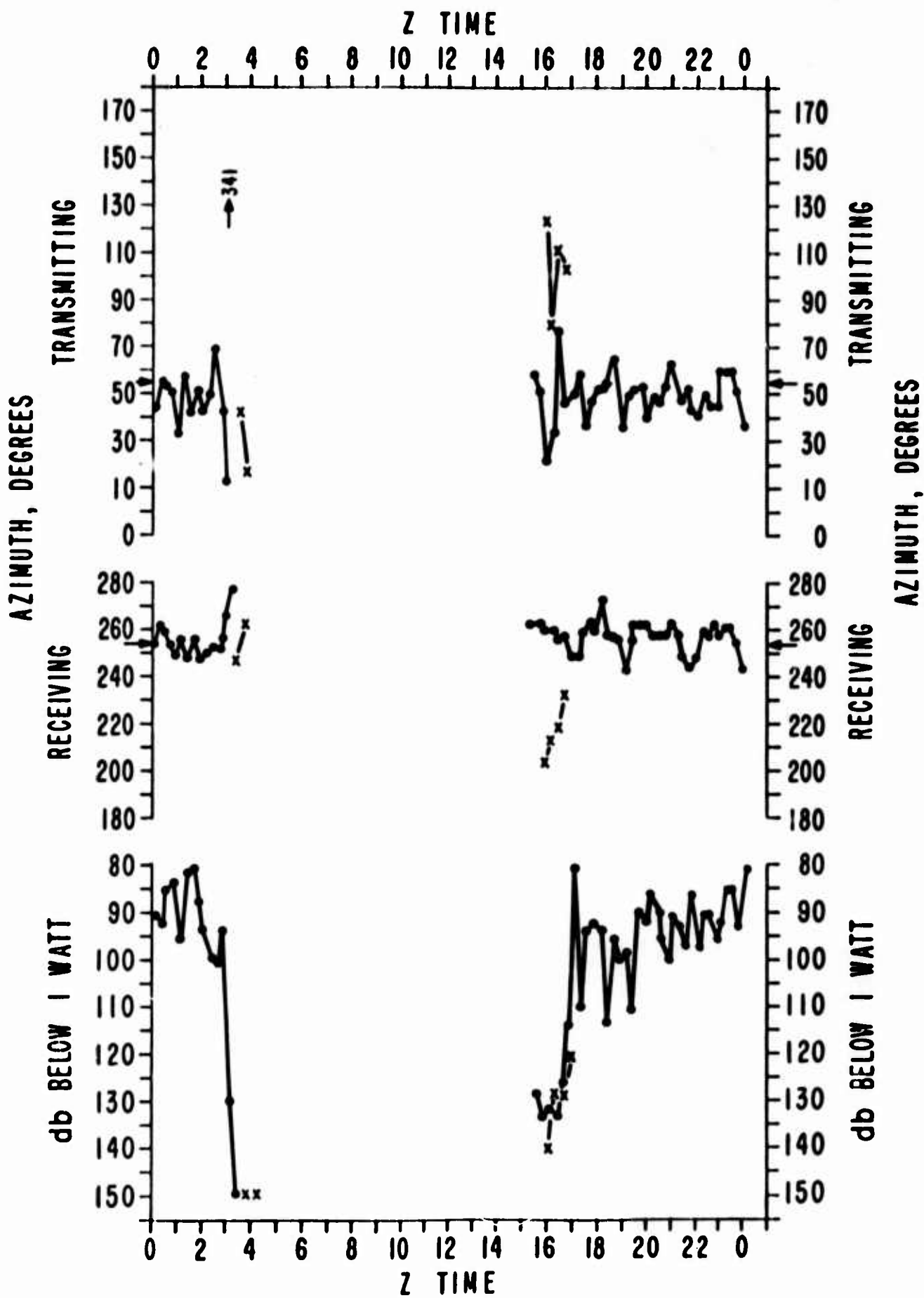
FIGURE 18a DIURNAL PLOTS KAUAI-PALO ALTO 18 MC, 19 OCTOBER 1962
