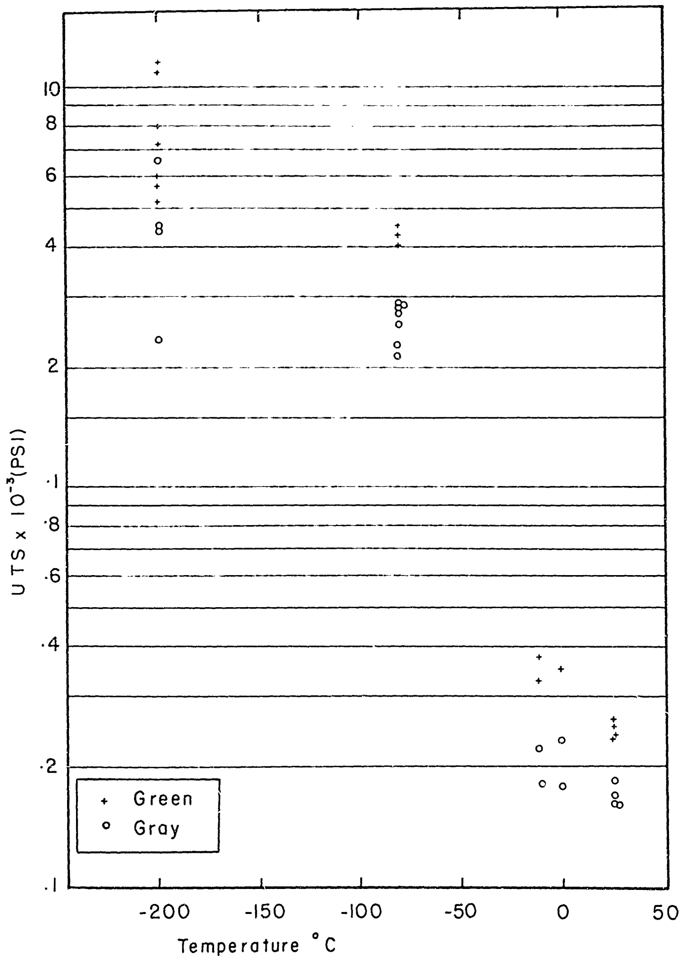
Fig. 2.4 - U.T.S. vs. temperature
