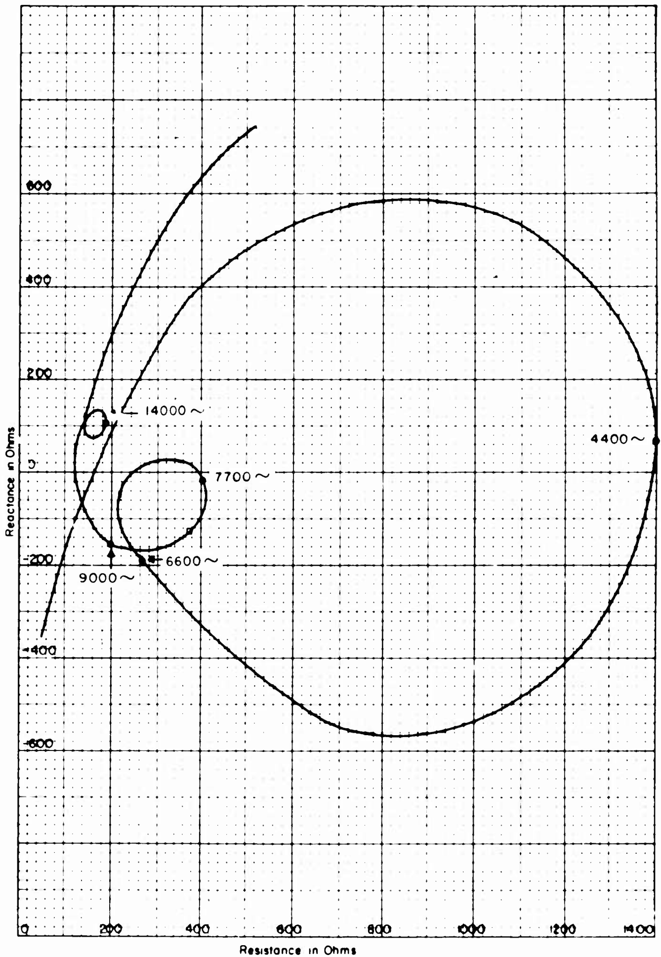
Figure 105 - Impedance Circle - 12 Ring Array - 1-3 4 inch Separation Between Rings
