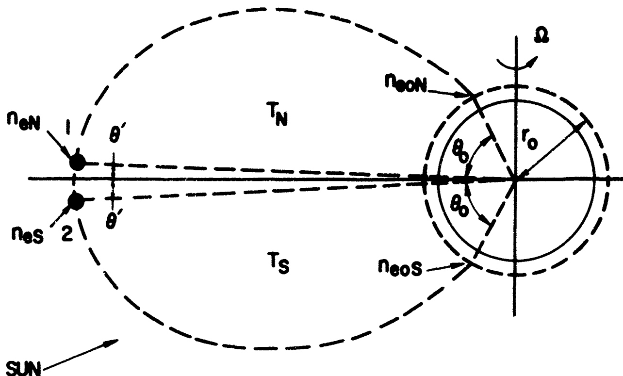
FIG. 6. PARAMETERS USED TO CALCULATE R_{00} AT THE REFERENCE LEVEL AT TWO MAGNETICALLY CONJUGATE POINTS WHEN THE TEMPERATURE IN THE NORTHERN AND SOUTHERN HEMISPHERES ARE DIFFERENT BUT CONSTANT IN EACH HEMISPHERE.
