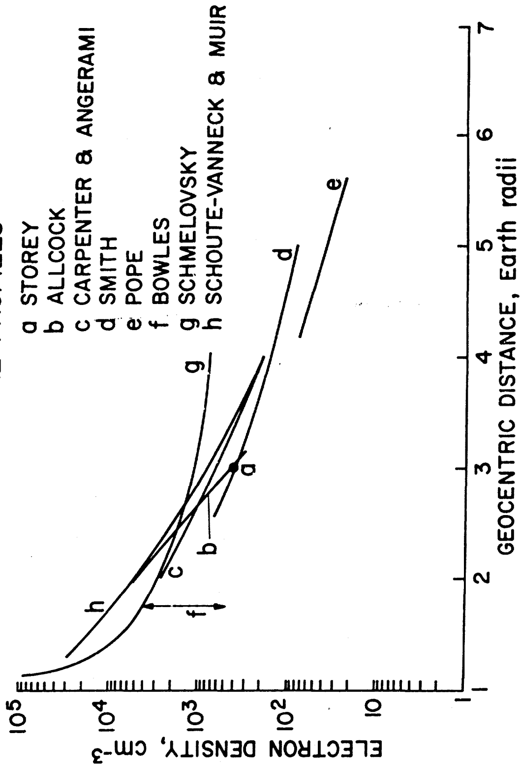
FIG. 19b. EXAMPLES OF EXPERIMENTAL OBSERVATIONS OF EXOSPHERIC ELECTRON DENSITY (EQUATORIAL PROFILES).
