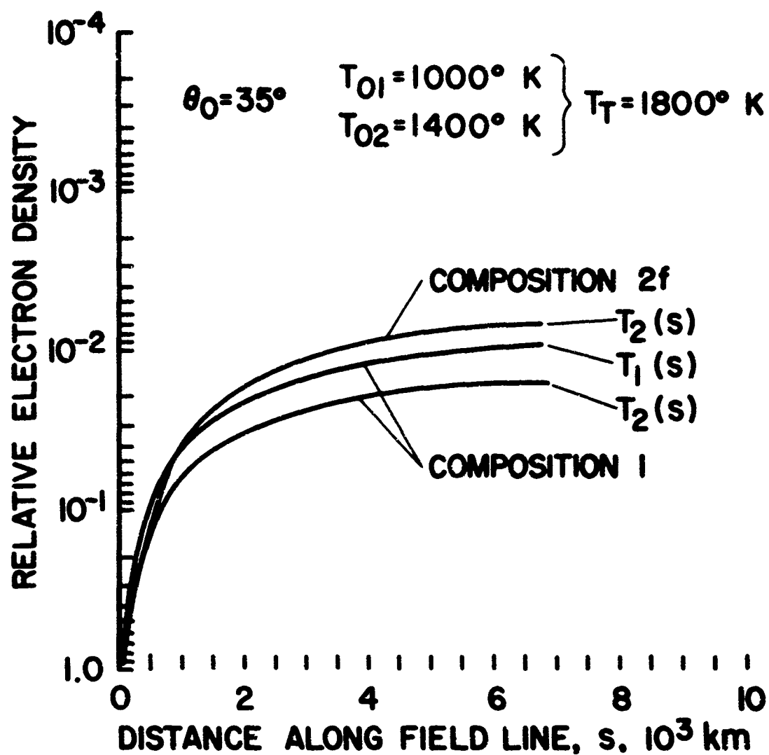
FIG. 14a. TO ILLUSTRATE, FOR A NON-ISOTHERMAL EXOSPHERE (SEE FIG. 13), THE RELATIVE ELECTRON DENSITY DISTRIBUTION ALONG A FIELD LINE WITH FEET (AT 500 KM ABOVE THE EARTH) AT GEOMAGNETIC LATITUDE 35^\circ (SEE TABLES 1 AND 2).
