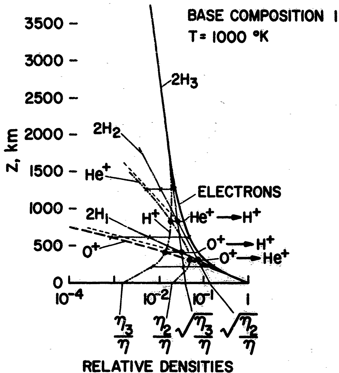
FIG. 9b. RELATIVE ELECTRON AND ION DENSITIES AS A FUNCTION OF THE GEOPOTENTIAL HEIGHT, z , FOR AN ISOTHERMAL EXOSPHERE. Comparison with Fig. 9c indicates the effect on the distributions of changing the temperature only.
