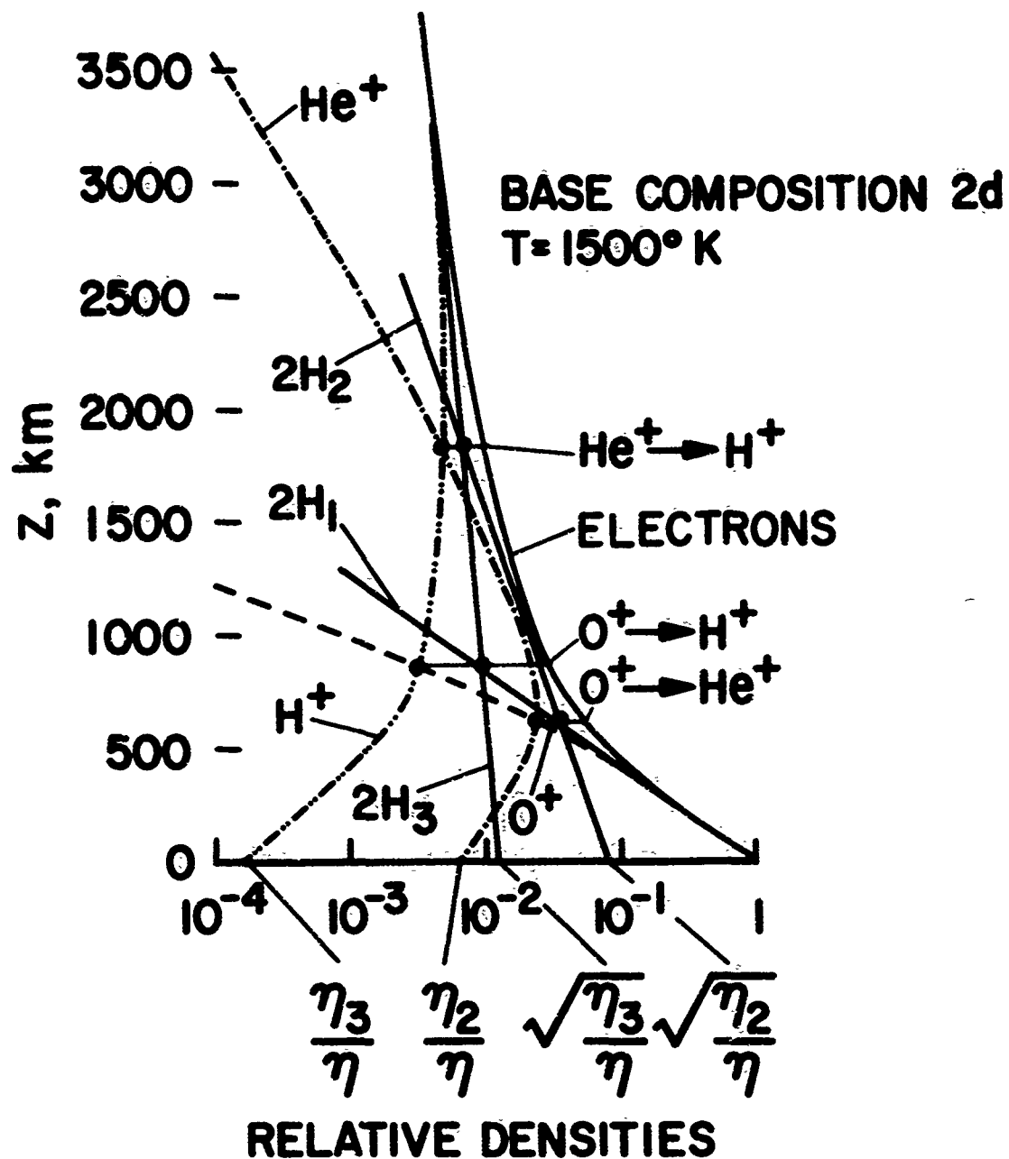
FIG. 9d. RELATIVE ELECTRON AND ION DENSITIES AS A FUNCTION OF THE GEOPOTENTIAL HEIGHT, z , FOR AN ISOTHERMAL EXOSPHERE. Comparison with Fig. 9c reveals the effect of changing the base composition only.
