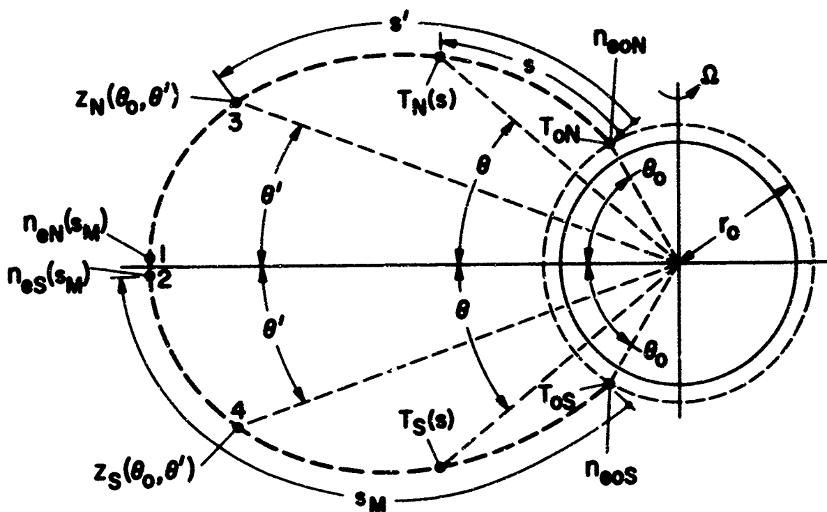
FIG. 7. PARAMETERS USED TO CALCULATE R_{00} AT THE REFERENCE LEVEL AT TWO MAGNETICALLY CONJUGATE POINTS WHEN THE TEMPERATURE IS TAKEN AS A CONTINUOUS FUNCTION T_N(s) IN THE NORTHERN HEMISPHERE, AND T_S(s) IN THE SOUTHERN HEMISPHERE. At points 1 and 2, the temperatures are the same.
