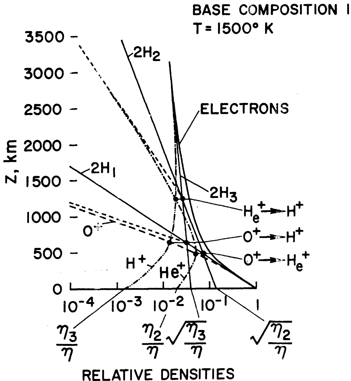
FIG. 9c. RELATIVE ELECTRON AND ION DENSITIES AS A FUNCTION OF THE GEOPOTENTIAL HEIGHT, z , FOR AN ISOTHERMAL EXOSPHERE. Comparison with Fig. 9b indicates the effect on the distributions of changing the temperature only. Comparison with Fig. 9d reveals the effect of changing the base composition only.
