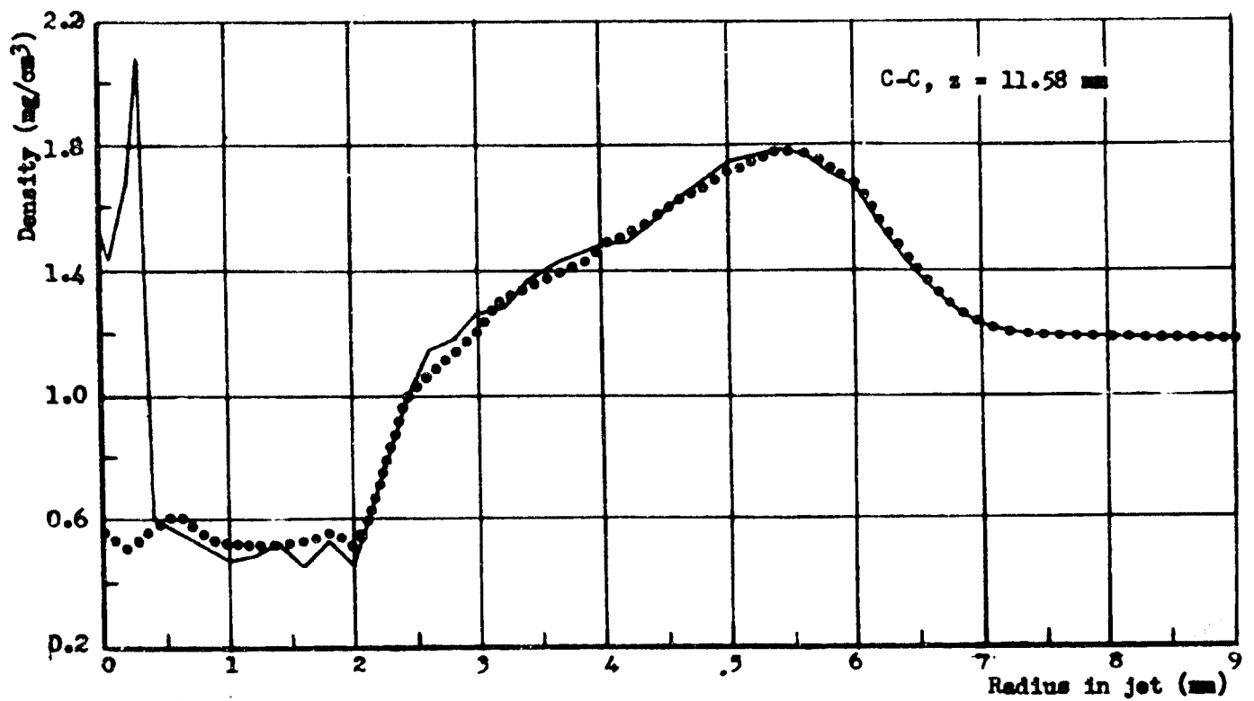
Figure 6 - Density cross sections with probe; —, jet + probe; ..... , jet without probe.
