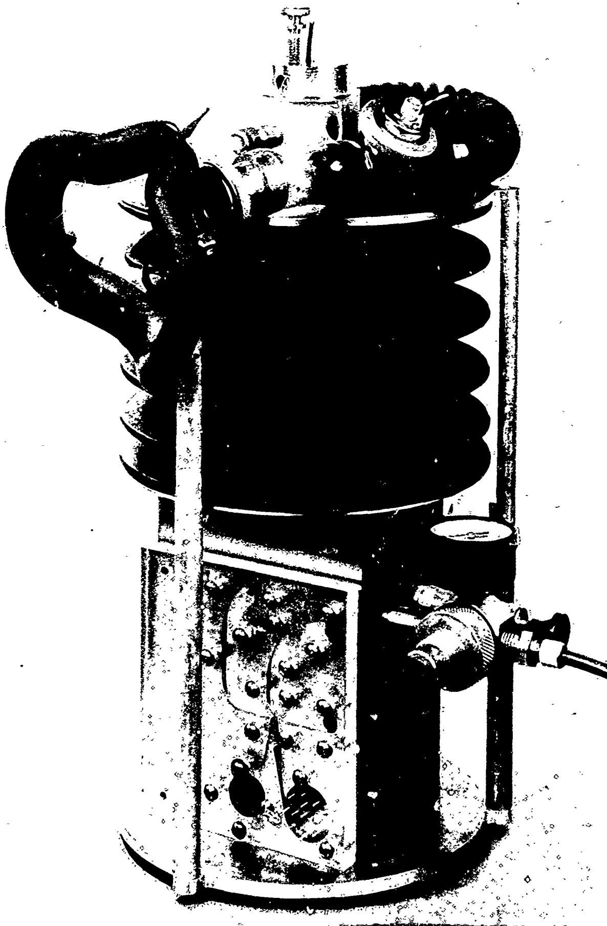
Figure 2. Volume-limited fluid amplifier respirator.
