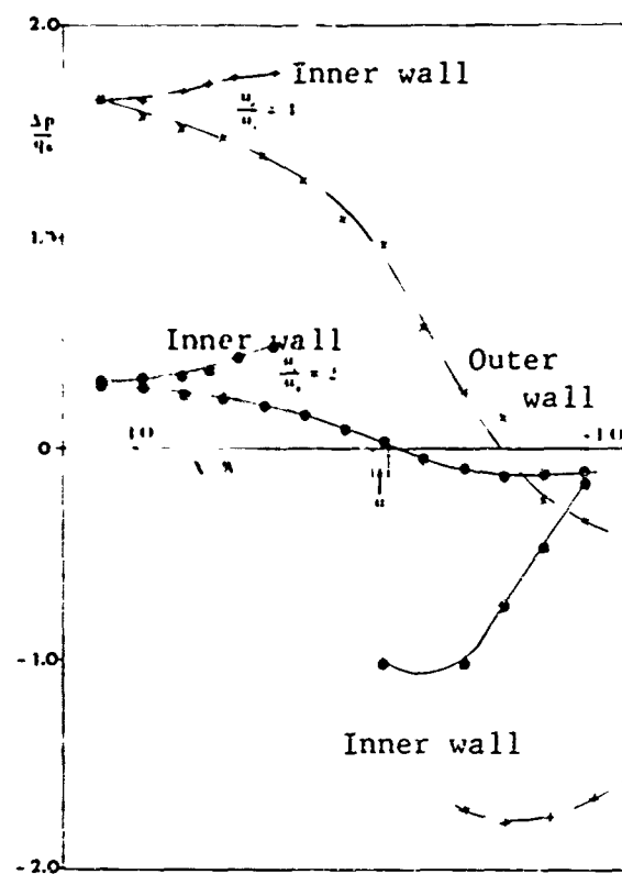
Fig. 11. Pressure distribution with injection, straight channel R = 1.0
