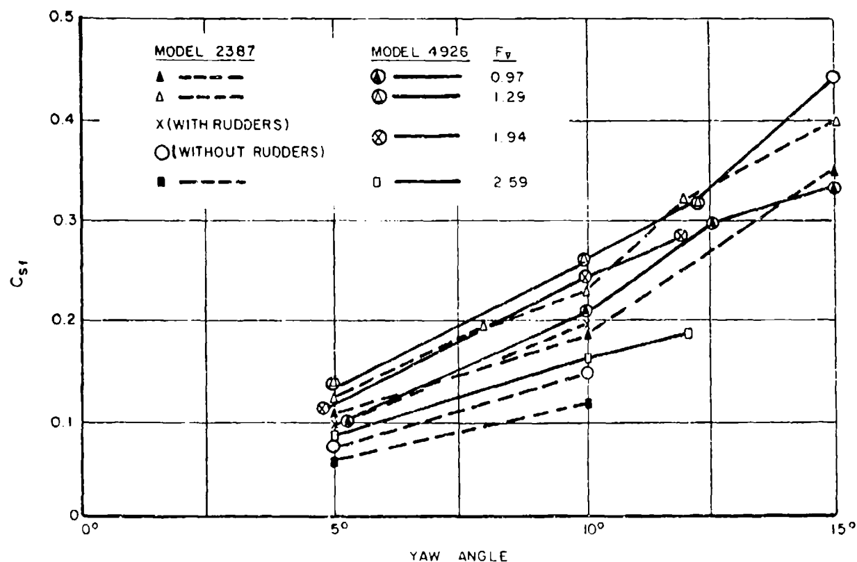
FIGURE 38. SIDE FORCE COEFFICIENTS OF MODELS IN CALM WATER.
