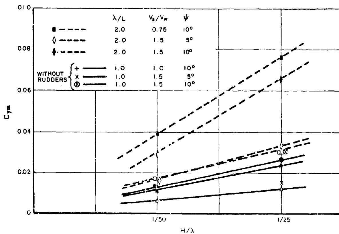
FIGURE 42. DOUBLE AMPLITUDES OF YAW MOMENT IN WAVES.
