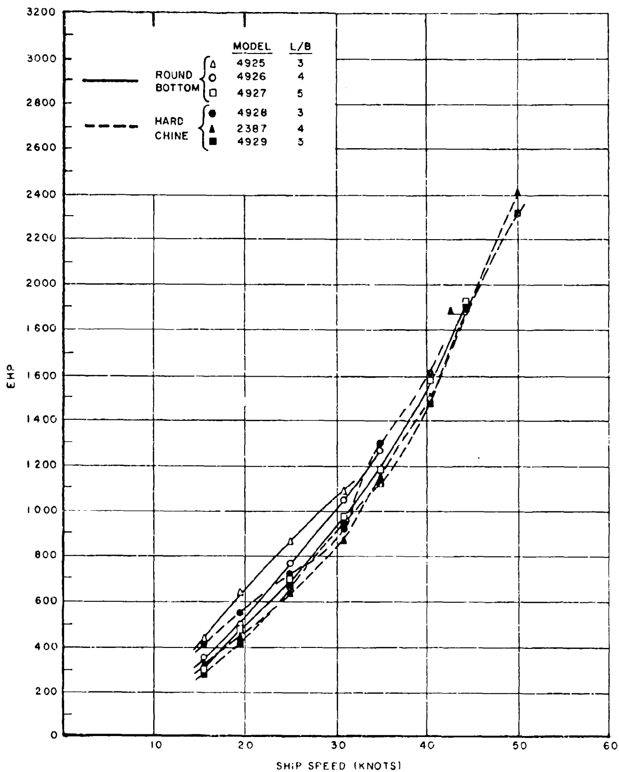
FIGURE 17. EHP IN AHEAD SEA STATE 3
