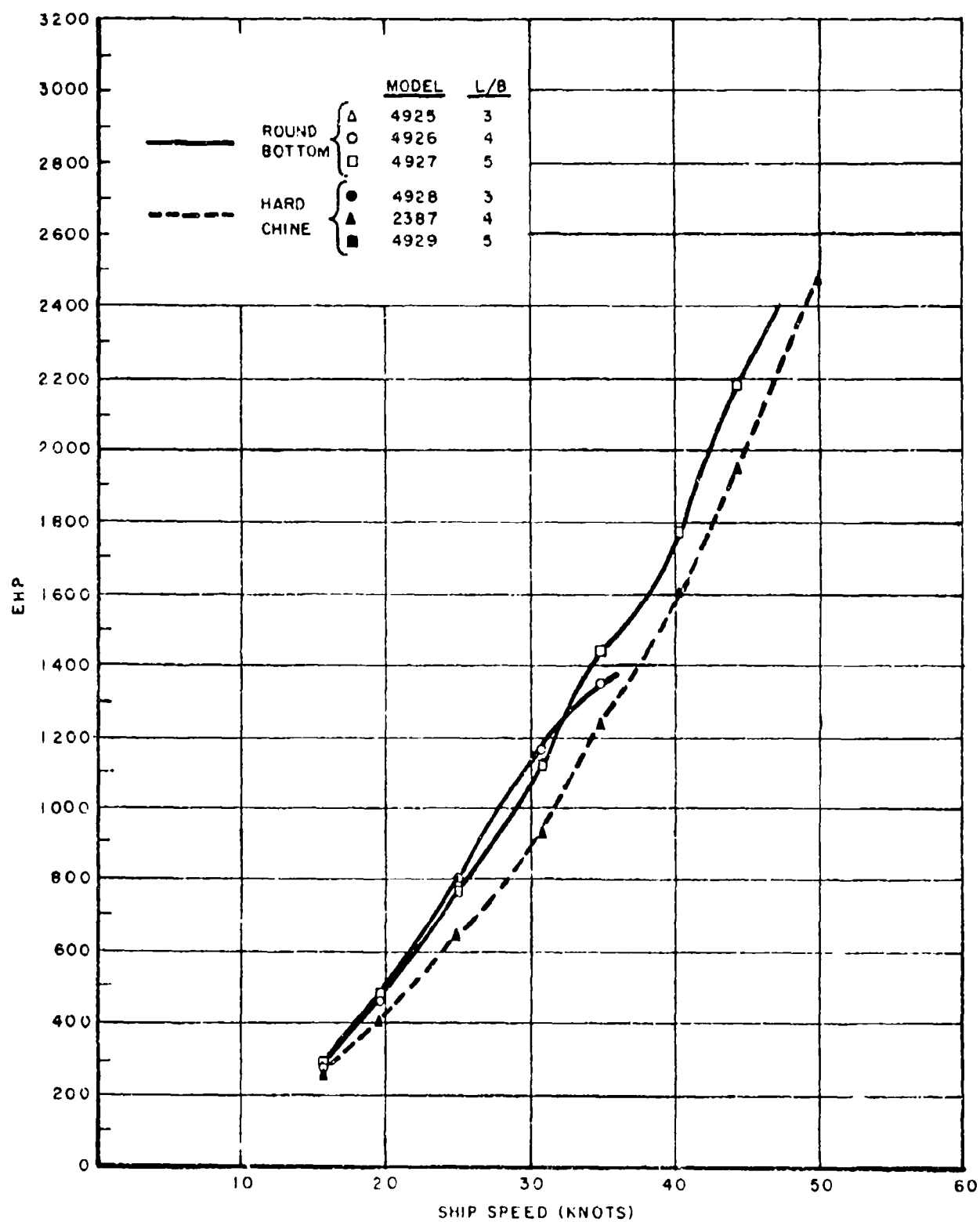
FIGURE 18. EHP IN FOLLOWING SEA STATE 3
