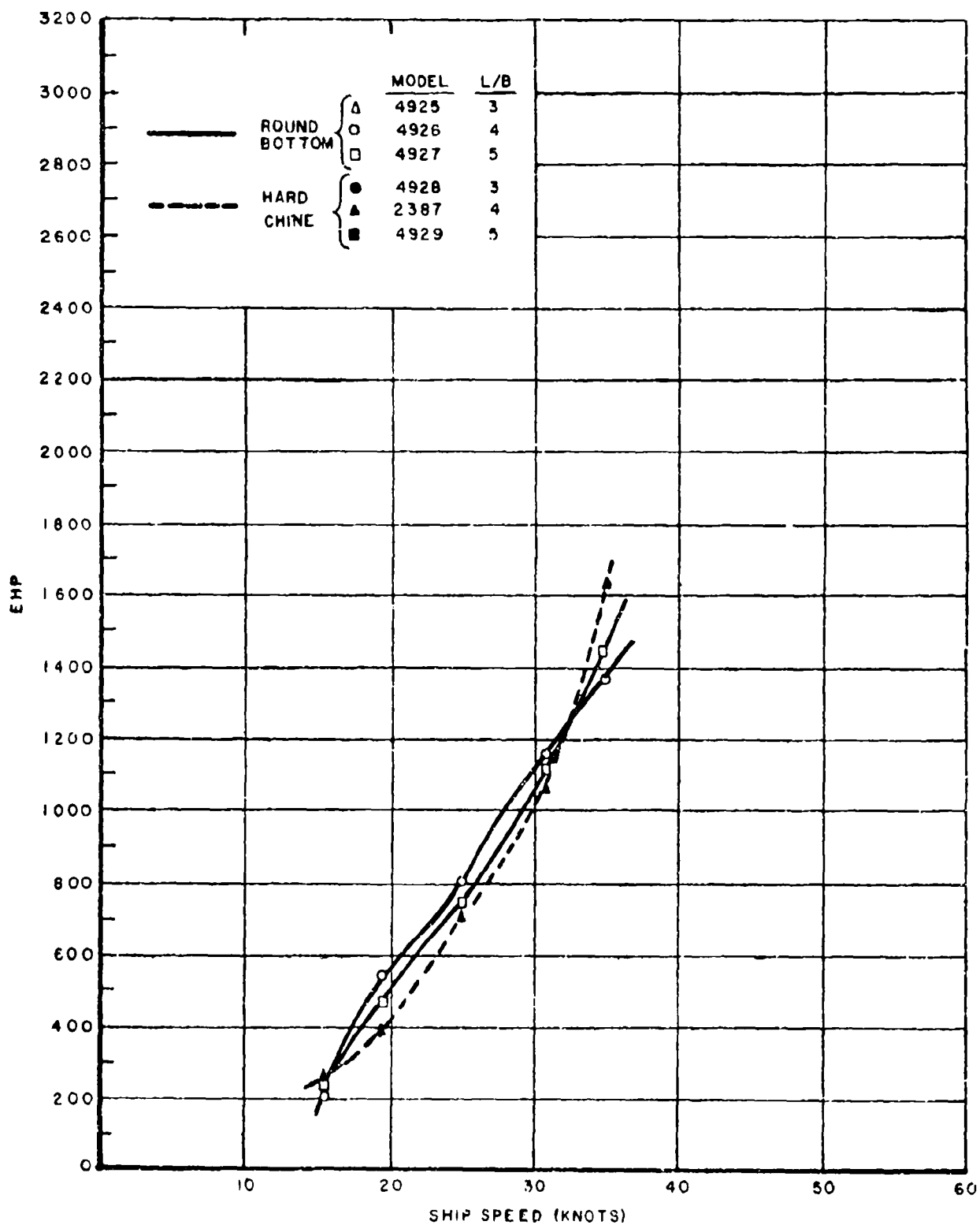
FIGURE 20. EHP IN FOLLOWING SEA OF STATE 5
