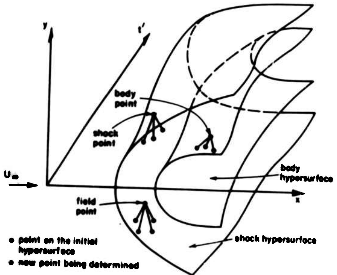
Figure 12 Representation of the basic elements of the numerical integration procedure.
