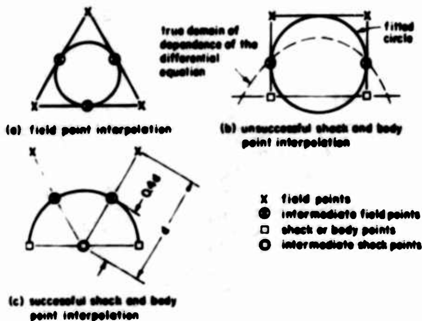
Figure 20 Interpolation schemes used by PATCH in the initial surface.
