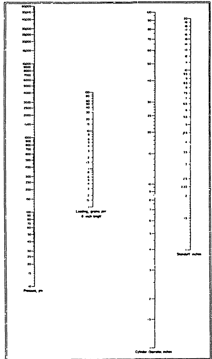
UNDERWATER SHOCK PRESSURE FOR LINE CHARGES OF PETN EXPLOSIVES (FOR OTHER EXPLOSIVES USE TNT EQUIVALENT/125 = LOADING)
