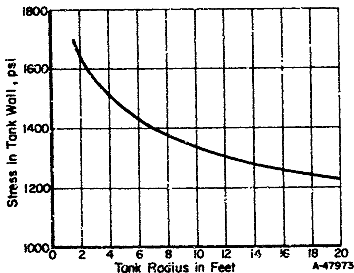
FIGURE 8. TANK WALL STRESS VERSUS DISTANCE FROM CHARGE
