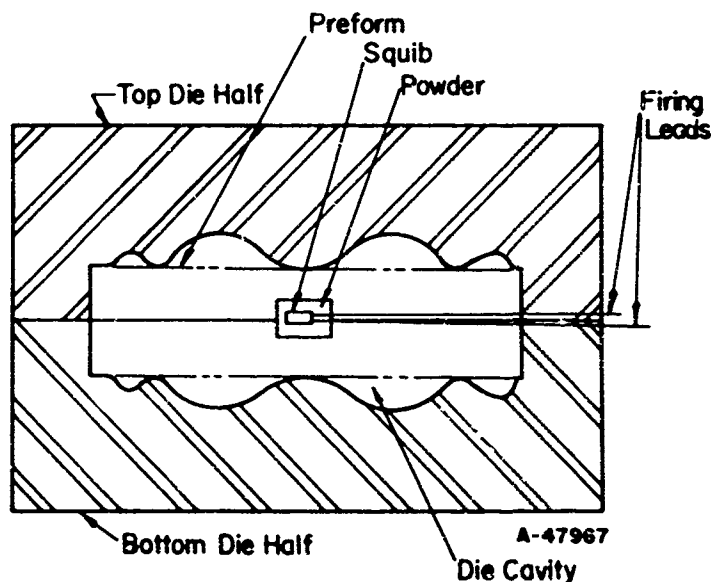
FIGURE 1. CONFINED SYSTEM OF EXPLOSIVE FORMING (5)
