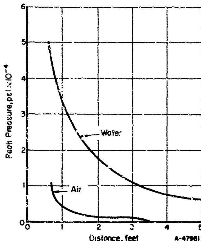
FIGURE 21. PEAK PRESSURE VERSUS DISTANCE (33)
