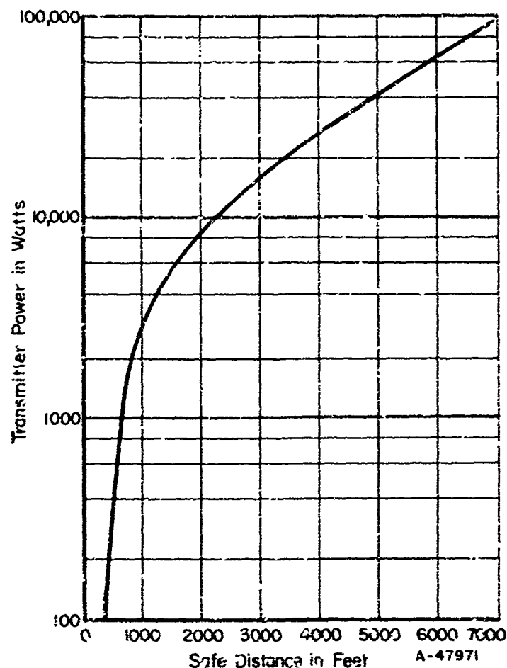
FIGURE 4. TRANSMITTER POWER VERSUS SAFE EXPLOSIVE OPERATING DISTANCE(20)
