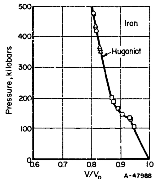
FIGURE 50. HUGONIOT CURVE FOR IRON (53)
