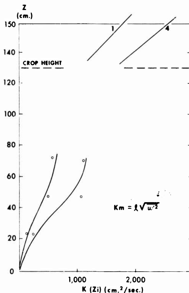
FIGURE 26.—Transfer coefficient for momentum ( K_m ) as a function of height ( z ) in and above a wheat crop, July 23, 1960.
