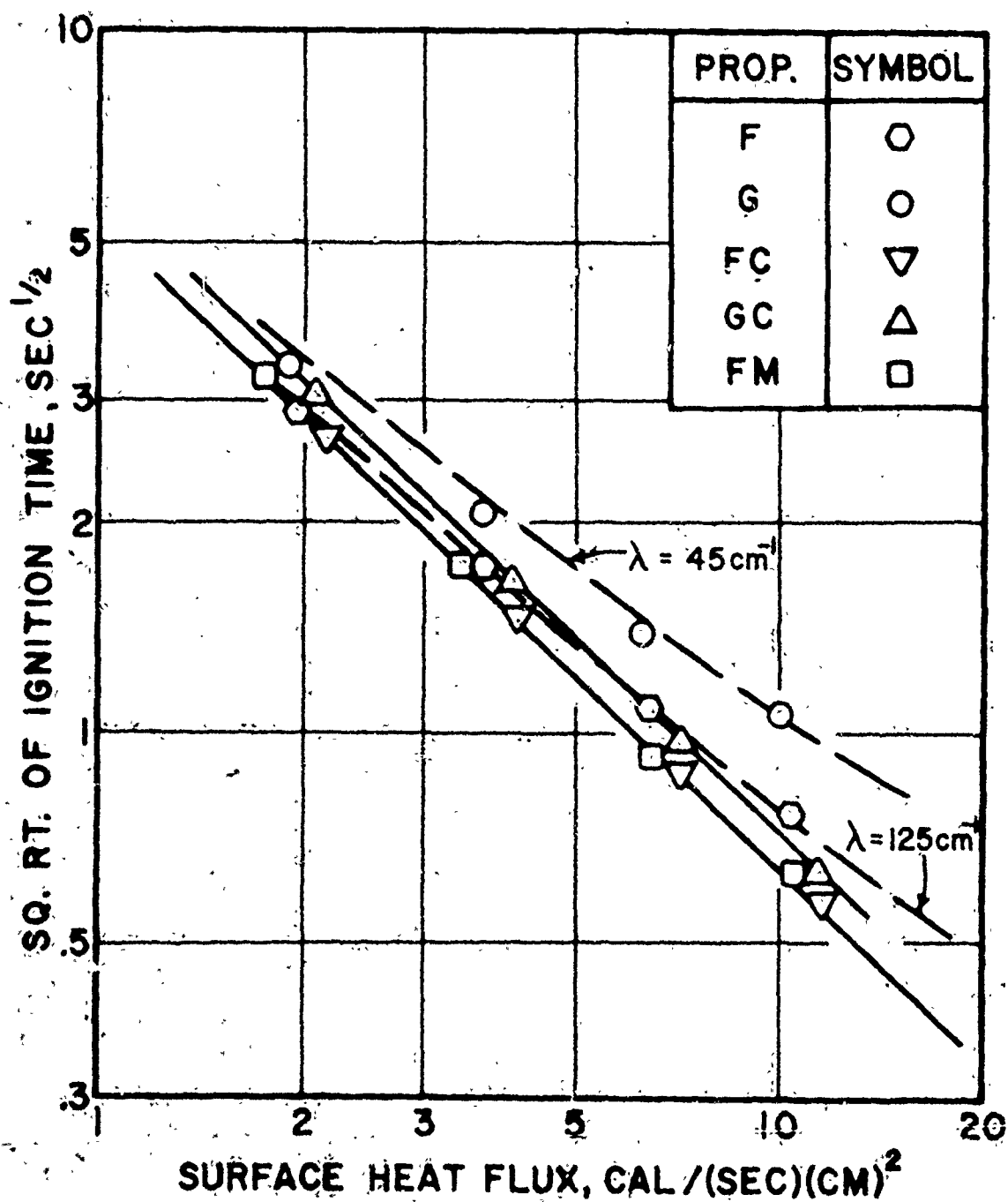
Figure 8. The Effect of Solid Transmissivity on Propellant Ignition Times. The opacity values of 45 \text{ cm}^{-1} and 125 \text{ cm}^{-1} are best fit values for the G and F propellants respectively.
