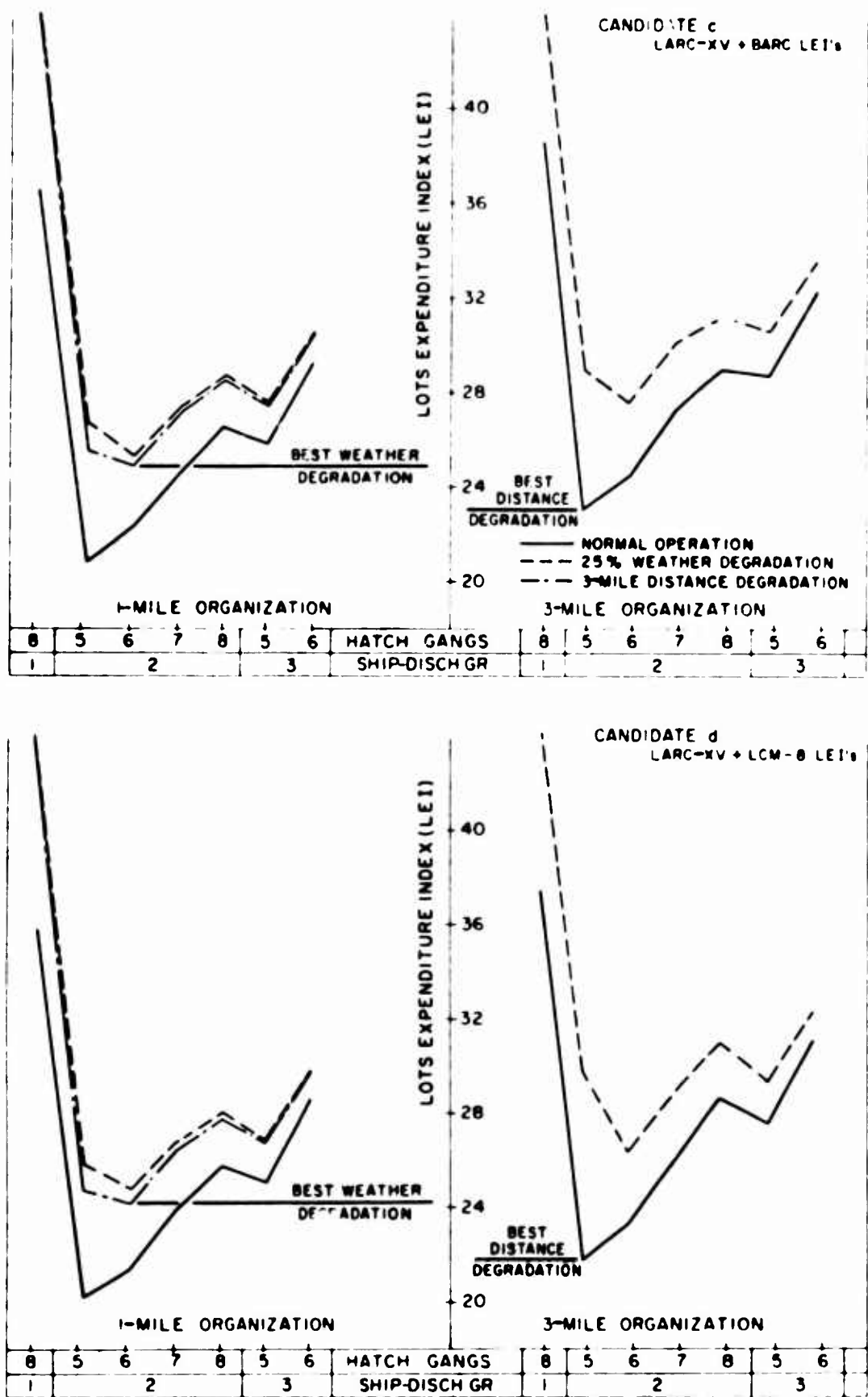
Figure 10. Normal and Degradation LEI's for LOTS System Candidates (Sheet 2 of 4)
