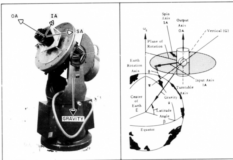
Figure 1. Tumbling Test.
