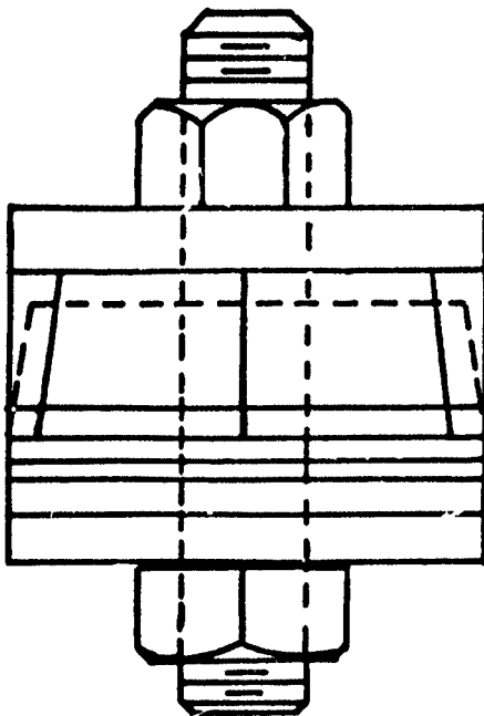
CROSS-SECTIONAL VIEW OF ASSEMBLED PACKING
