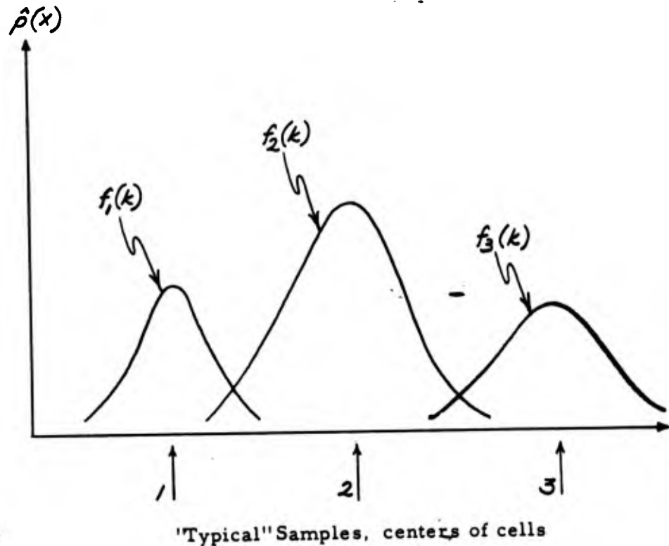
Fig. II-2. Local References of a Probability Density
