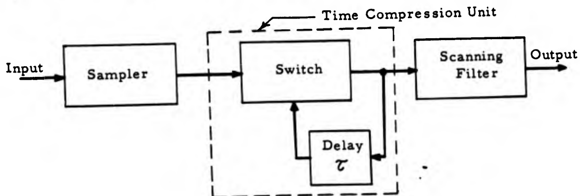
Fig. III-1. A DELTIC Spectrum Analyzer
