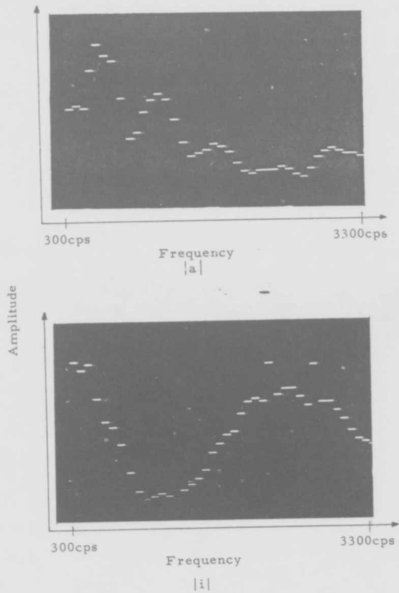
Fig. 7. Short Term Digitized Energy Density Spectra for the Vowel Sounds |a| and |i| .
