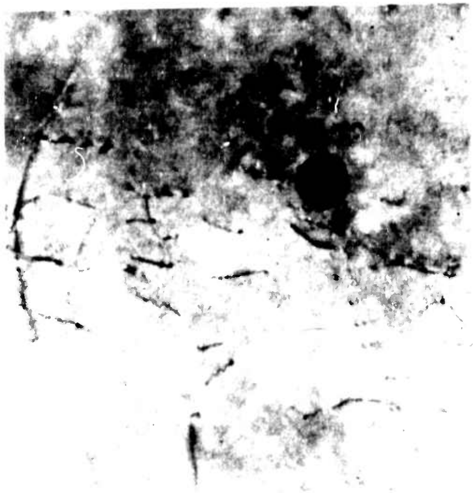
Figure 18 - A larger inclusion particle acting as dislocation source. (Techiney flake beryllium). 40,000:1.
