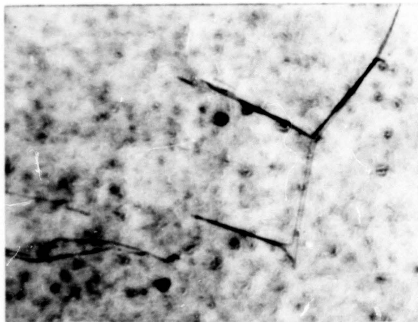
Figure 46 - Dipole formation in high purity specimen. 40,000:1.
