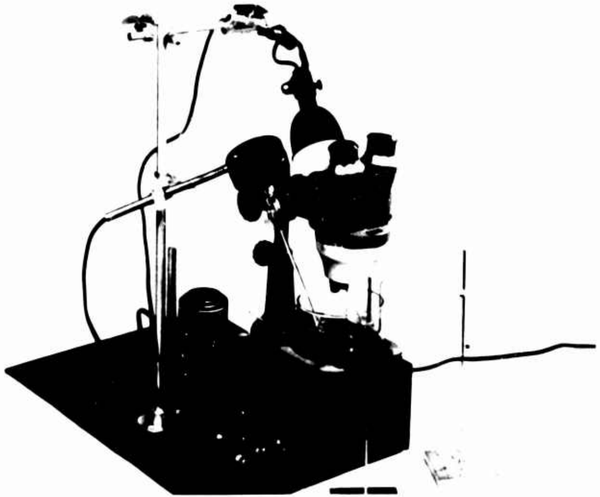
Figure 1 - Electropolishing apparatus used for the preparation of thin specimens for transmission electron microscopy. ("Slow" method).
