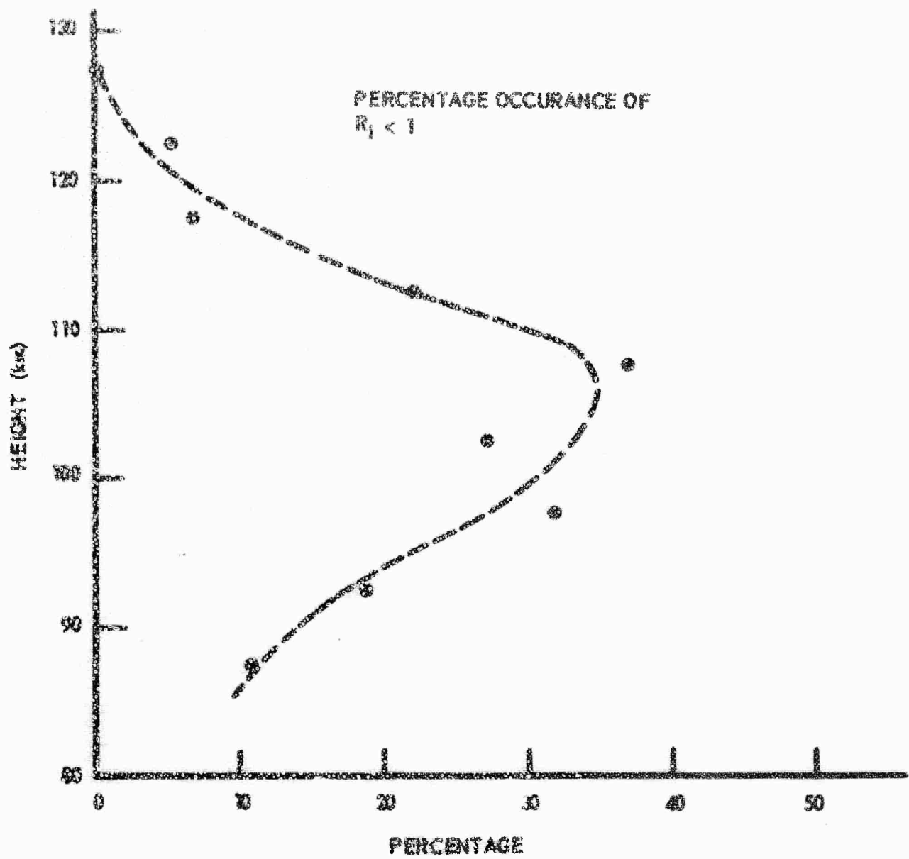
Figure 14. Percentage Occurance of R_1 < 1 Versus Altitude.
