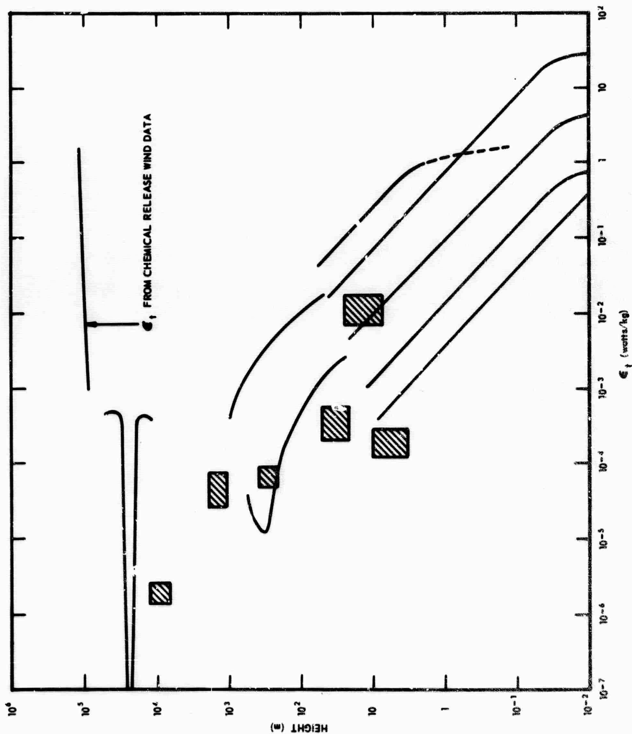
Figure 13. Viscous Energy Dissipation Rate from Altitudes of 1 cm to 110 km.
