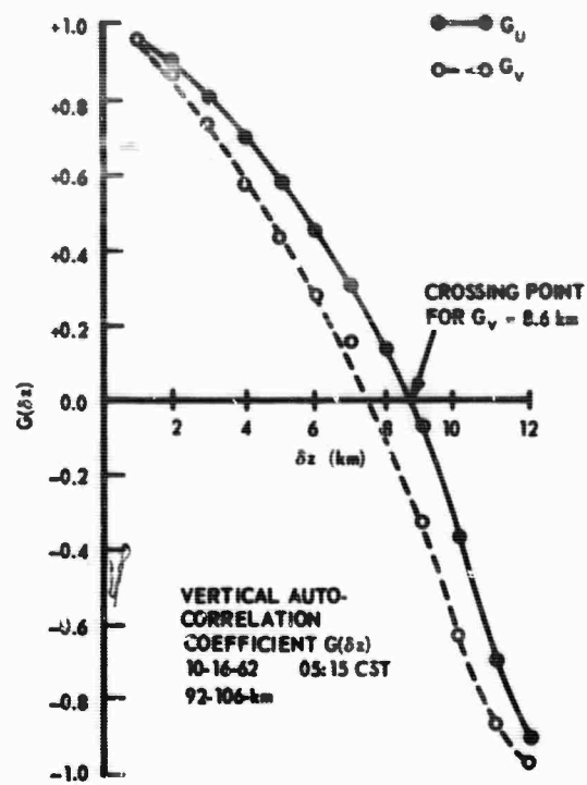
Figure 1. Typical Vertical Autocorrelation Curve.
