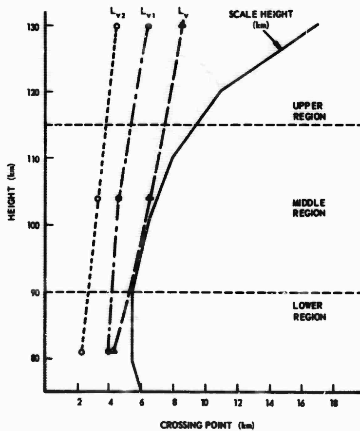
Figure 2. Vertical Autocorrelation Scales Versus Altitude.
