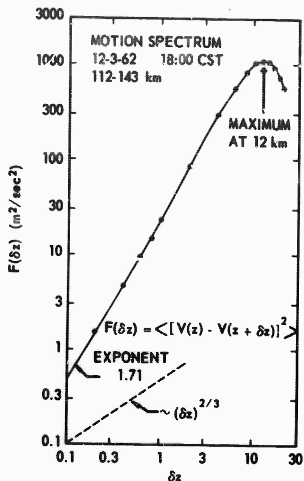
Figure 3. Typical Motion Spectrum Curve.
