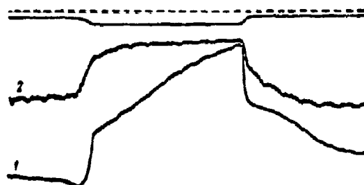
Fig. 6. Jump-like change in level of intracranial level of EPG (1) and intracranial pressure (2).
