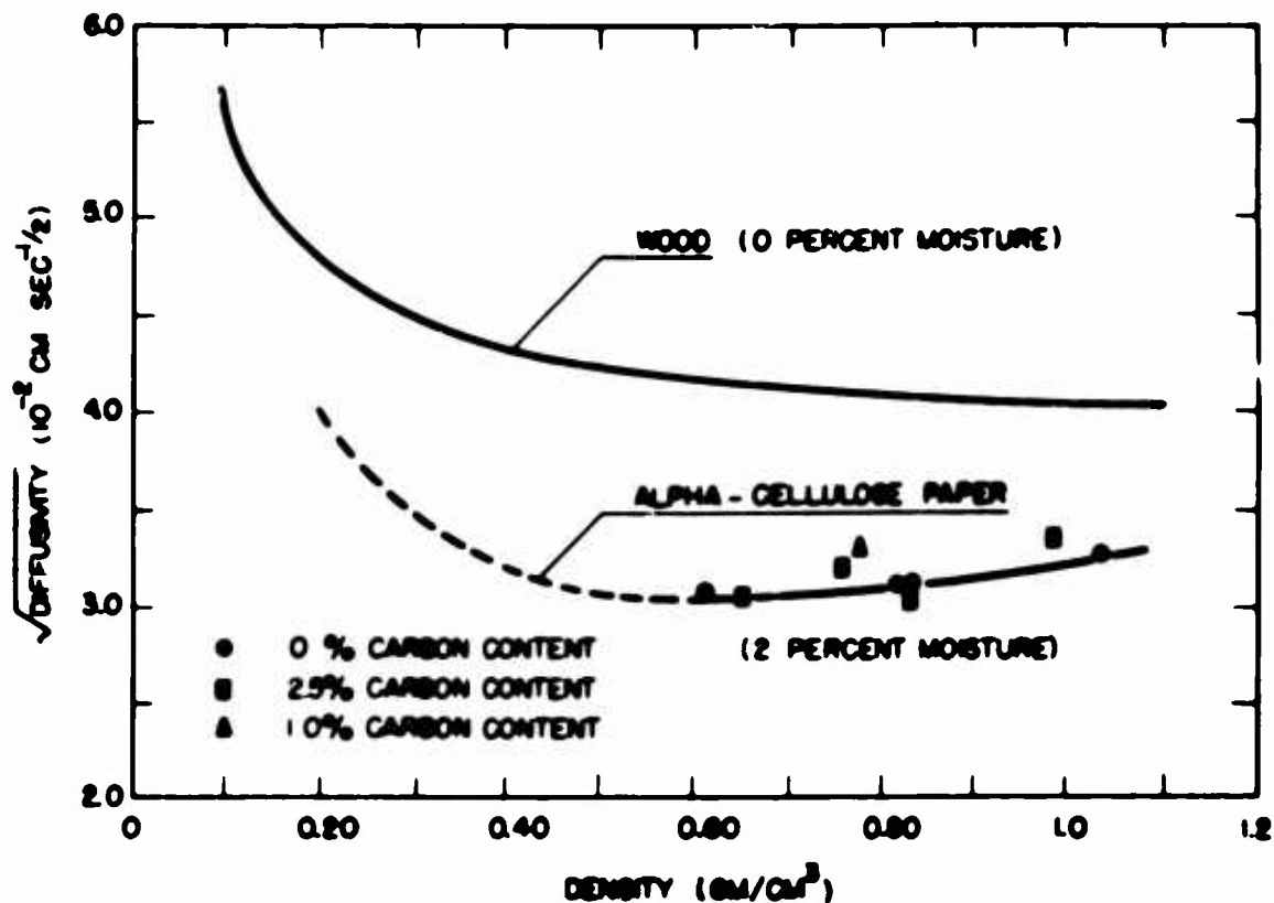
Figure 1.--Thermal diffusivity-density relationship for wood and alpha-cellulose paper
